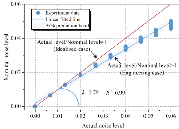
Figure 3: Relationship between the nominal noise level and the actual noise level.
