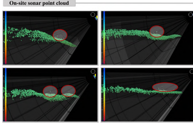
Figure 20: Sparse outlier noise deviating from the riverbed terrain, induced by aquatic vegetation or suspended particulates.
