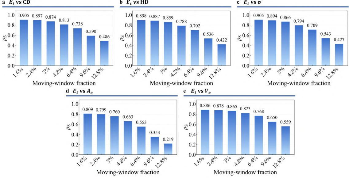
Figure 8: Sensitivity analysis of the equivalent thickness metric to the local window-size parameter. a. Correlation between equivalent thickness and Chamfer distance. b. Correlation between equivalent thickness and Hausdorff distance. c. Correlation between equivalent thickness and noise intensity. d. Correlation between equivalent thickness and area error. e. Correlation between equivalent thickness and volume error.
