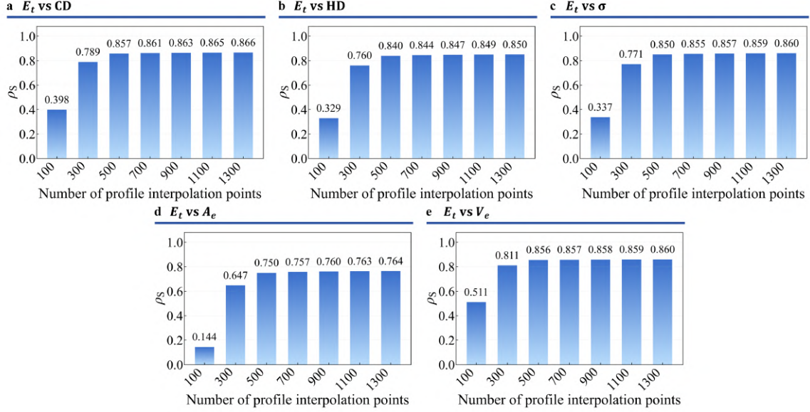
Figure 9: Sensitivity analysis of the equivalent thickness metric to the interpolation density parameter. a. Correlation between equivalent thickness and Chamfer distance. b. Correlation between equivalent thickness and Hausdorff distance. c. Correlation between equivalent thickness and noise intensity. d. Correlation between equivalent thickness and area error. e. Correlation between equivalent thickness and volume error.
