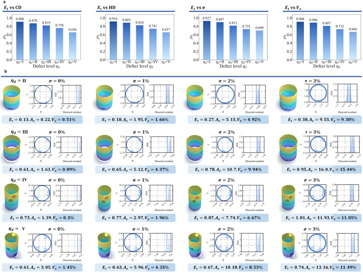
Figure 6: Morphological robustness analysis considering point clouds with local defects or structural damage. a. Comparison of correlations across different defect severity levels. b. Visualizations of point clouds containing defects or structural damage at different severity levels.
