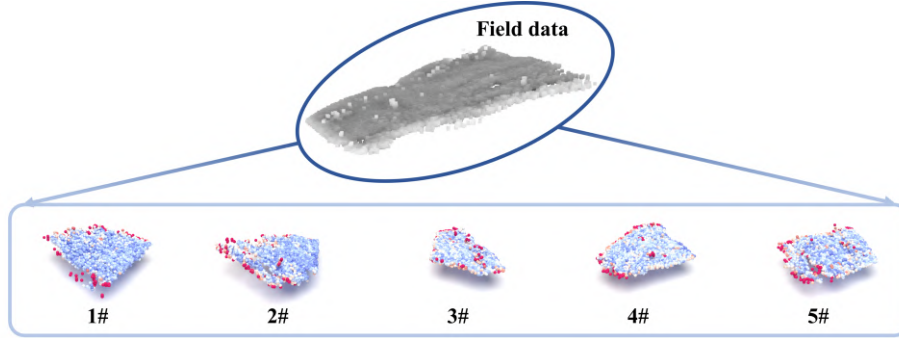
Figure 22: Visualization of N2P attention on representative noisy field sonar point cloud acquired in a turbid environment with dense aquatic vegetation.
