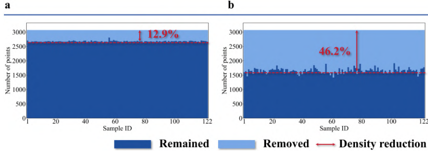
Figure 14: Effects of SOR and ROR on point-cloud density. a, Effect of SOR on point-cloud density. b, Effect of ROR on point-cloud density.
