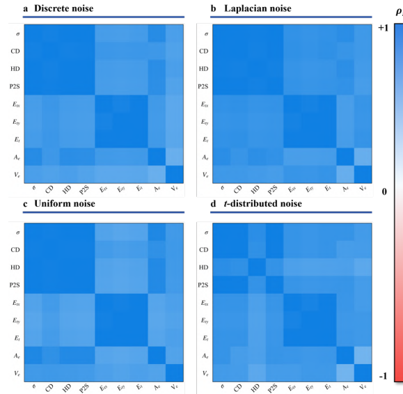
Figure 4: The noise generalization results of the equivalent thickness metric for underwater scour terrain inspection a. The noise generalization results under Discrete noise. b. The noise generalization results under Laplacian noise. c. The noise generalization results under Uniform noise. d. The noise generalization results under t-distributed noise.
