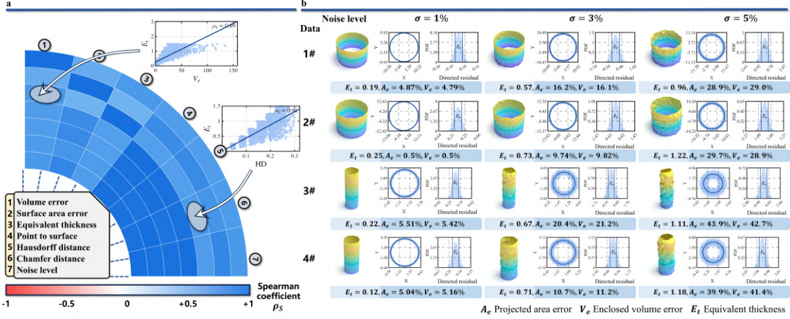
Figure 1: Validation of the proposed equivalent thickness metric. a Correlation analysis among all experimental metrics. b Visualisation of representative results from the experiments.
