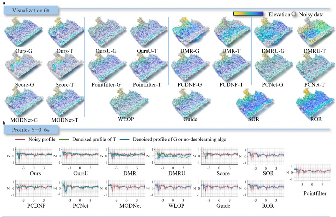
Figure 27: On-site performance and generalization comparison experiments (6#): a. Qualitative visualization on a representative sample; b. Comparison of the central Y-profile for the representative sample.
