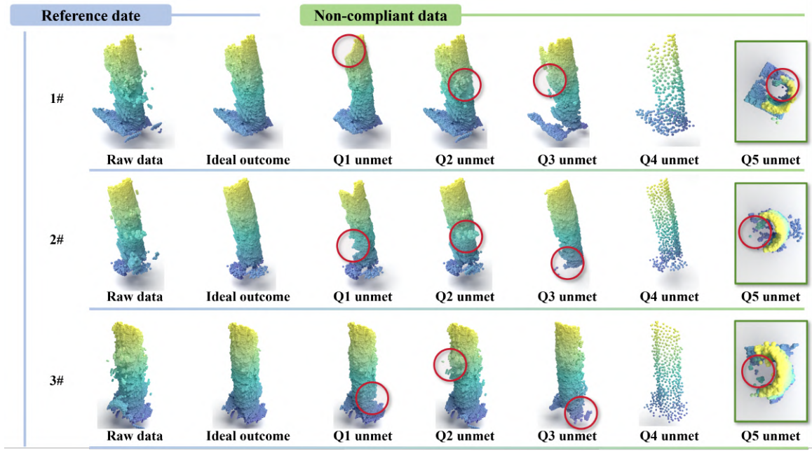
Figure 10: Representative quality-control examples that failed to satisfy each quality criterion
