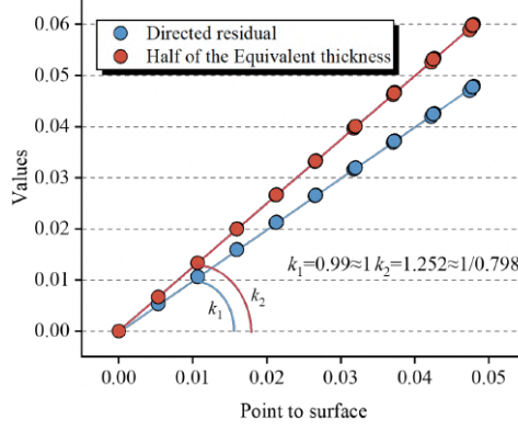
Figure 2: Relationship between equivalent thickness, directional residuals, and P2S.
