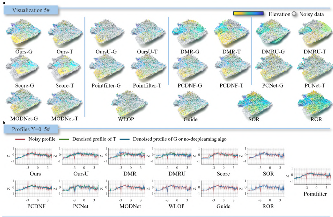
Figure 26: On-site performance and generalization comparison experiments (5#): a. Qualitative visualization on a representative sample; b. Comparison of the central Y-profile for the representative sample.
