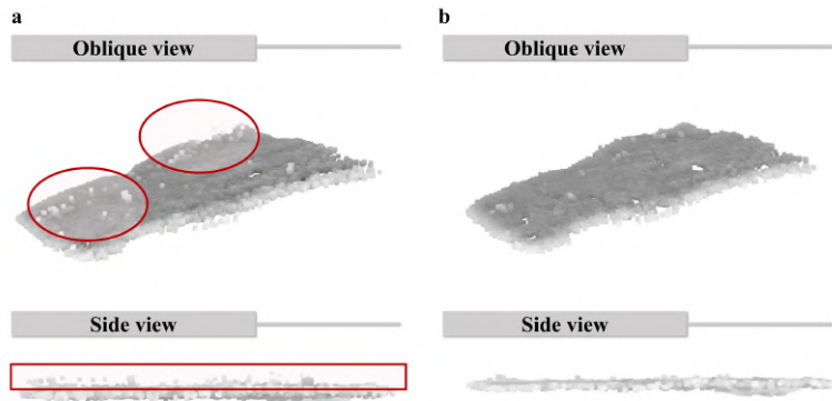
Figure 21: Unsupervised denoising results of SIREND-Net on representative field sonar point clouds acquired in a turbid environment with abundant aquatic vegetation. a. Before denoising; b. After denoising.
