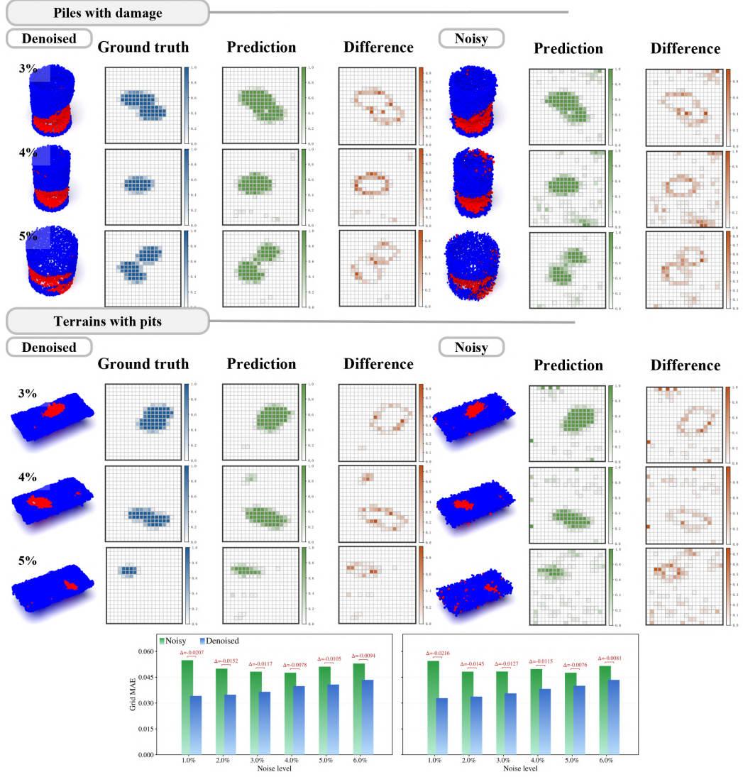
Figure 15: Quantitative evaluation of denoising for downstream tasks. a. Grid MAE results for pile point clouds with defects. b. Grid MAE results for terrain point clouds with scour.
