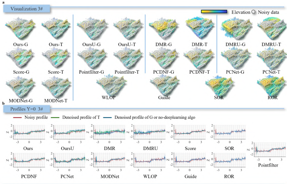
Figure 24: On-site performance and generalization comparison experiments (3#): a. Qualitative visualization on a representative sample; b. Comparison of the central Y-profile for the representative sample.
