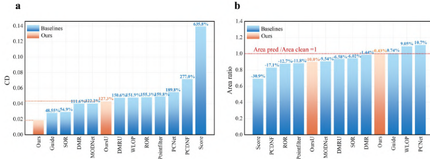
Figure 13: Quantitative comparison of extracted 2D boundaries after denoising under typical noise conditions. a. Chamfer distance between the extracted 2D boundary points from the clean and denoised point clouds. b. Enclosed area of the extracted 2D boundaries for the clean and denoised point clouds.
