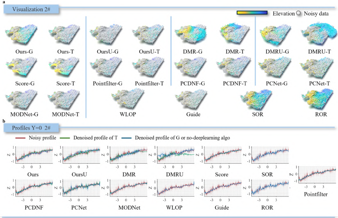
Figure 23: On-site performance and generalization comparison experiments (2#): a. Qualitative visualization on a representative sample; b. Comparison of the central Y-profile for the representative sample.
