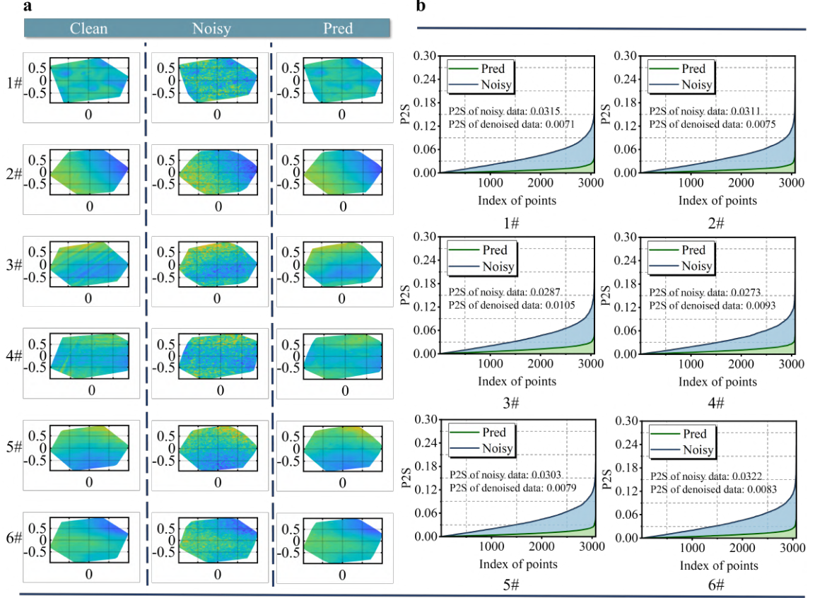
Figure 11: Extended qualitative results of numerical experiments under typical noise condition (4% Gaussian noise). a Comparison of horizontal projections before and after denoising. b Changes in P2S values of individual points before and after denoising, sorted in ascending order.
