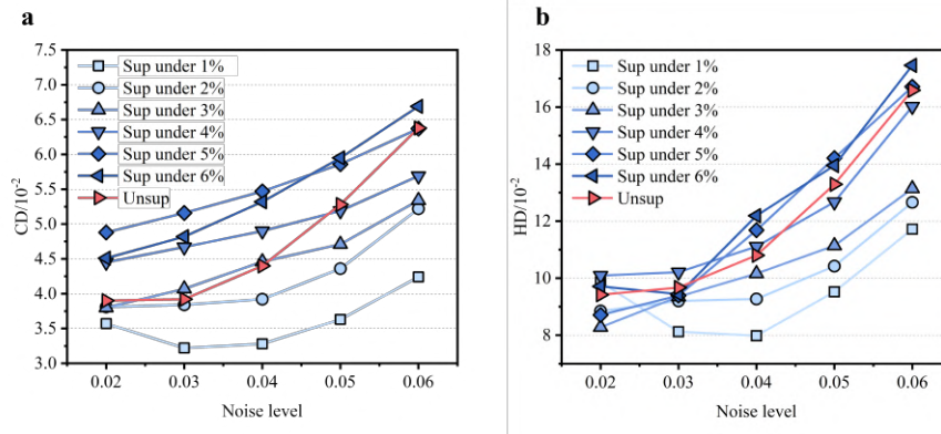
Figure 16: Results of the experiment on the supervised/unsupervised mode switching mechanism. a Chamfer distance results. b Hausdorff distance results.
