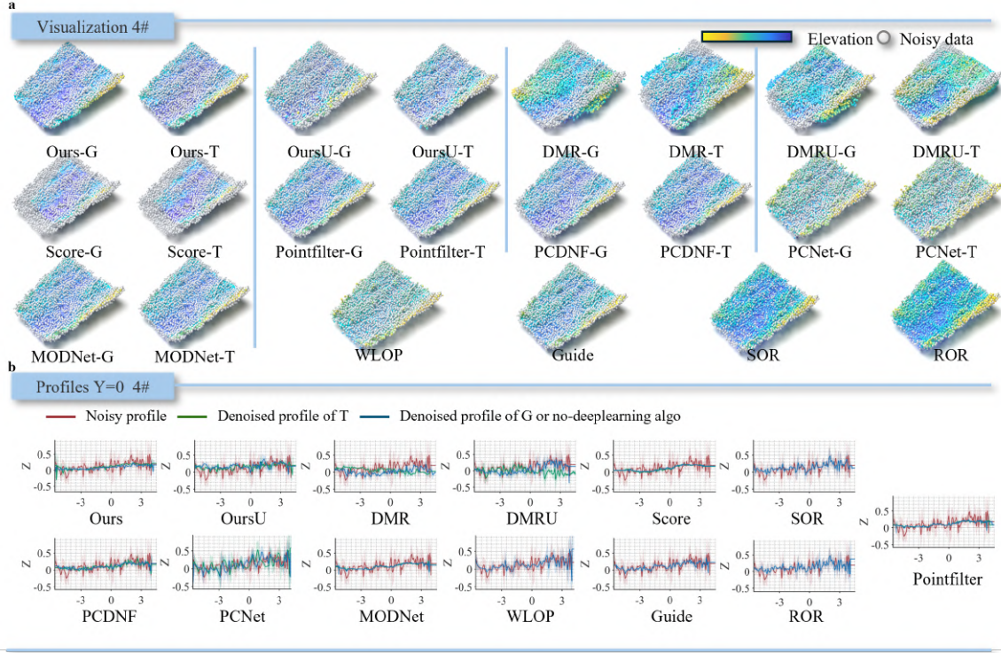
Figure 25: On-site performance and generalization comparison experiments (4#): a. Qualitative visualization on a representative sample; b. Comparison of the central Y-profile for the representative sample.
