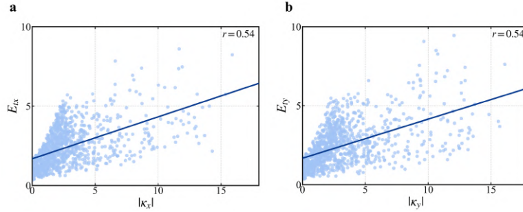
Figure 7: Curvature-based morphological robustness analysis. a Analysis results for the central profile along the X -direction. b Analysis results for the central profile along the Y -direction.
