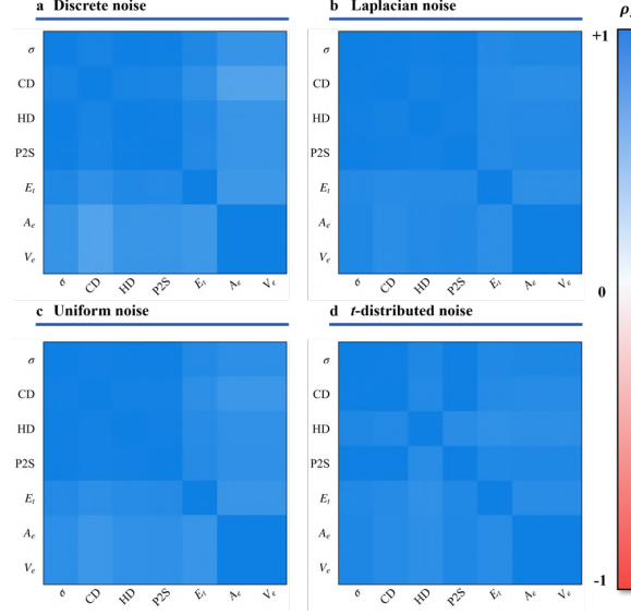
Figure 5: The noise generalization results of the equivalent thickness metric for underwater bridge foundation inspection. a. The noise generalization results under Discrete noise. b. The noise generalization results under Laplacian noise. c. The noise generalization results under Uniform noise. d. The noise generalization results under t-distributed noise.
