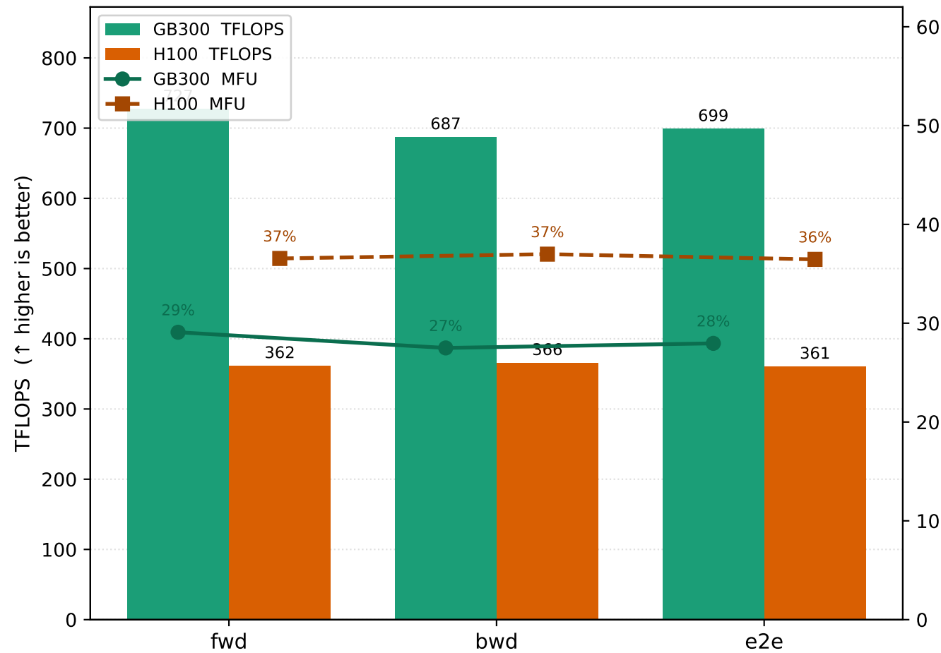
d128 (GB300 CUTLASS · H100 Hopper CUTLASS)
