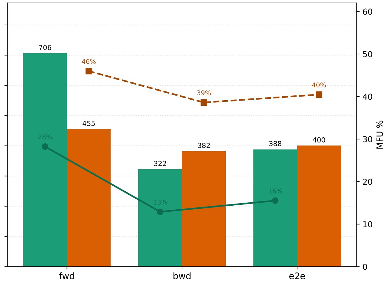
d256 (GB300 triton · H100 Hopper CUTLASS)
