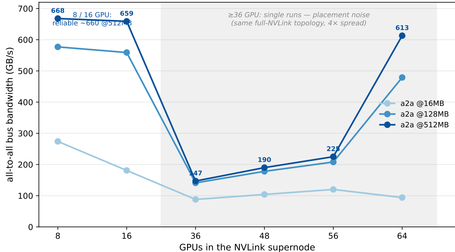
NVLink all-to-all is non-monotonic beyond 16 GPU — placement noise, not an N-scaling law
