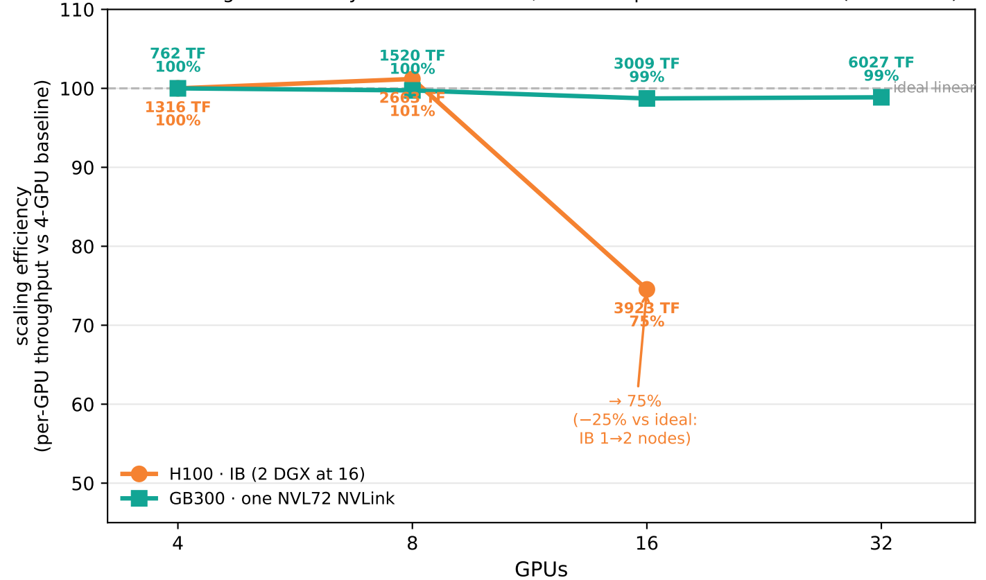
E2E scaling: GB300 stays flat over NVLink; H100 drops to 75% at 16 GPU (2 IB nodes)
