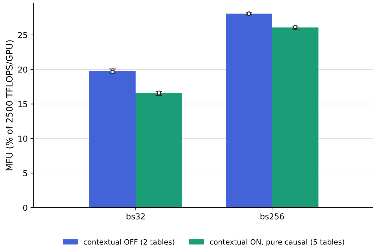
Matched A/B — identical settings, only contextual differs
