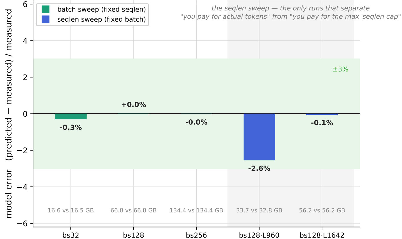
The law predicts every run to ≤2.6%
