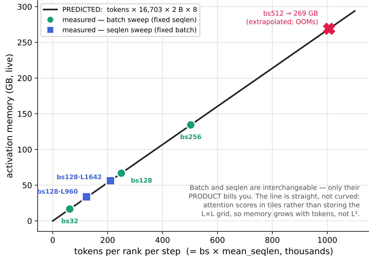
One law, two independent sweeps
