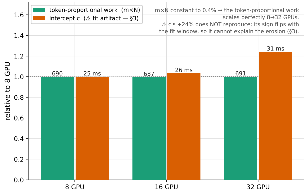
Weak scaling: the token-work is flat; c is a fit artifact
