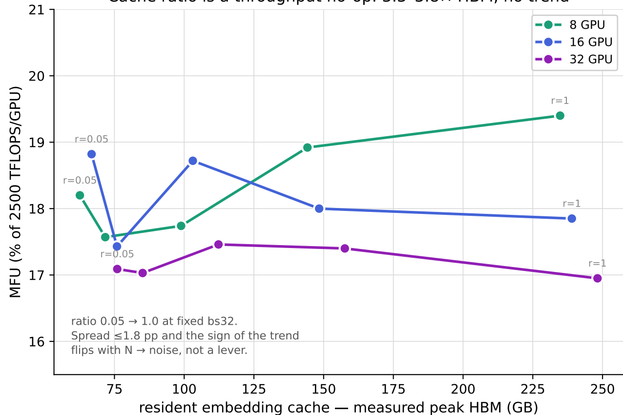
Cache ratio is a throughput no-op: 3.3-3.8x HBM, no trend
