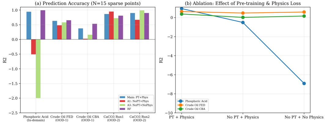
Figure 2: R^2 comparison across methods and sparsity levels. (a) Bar chart at N = 15 . (b) Ablation: pre-training vs. physics loss.
