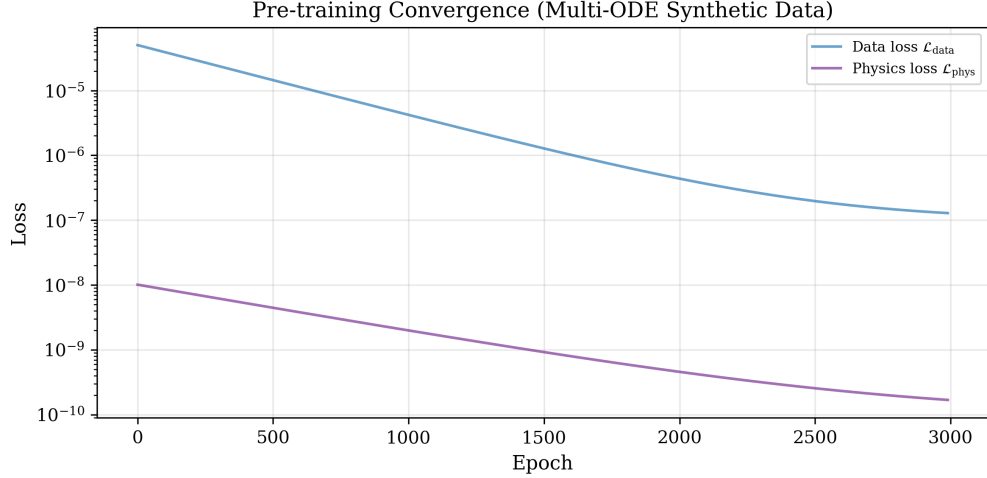
Figure 1: Pre-training convergence curves. Data loss and physics loss decrease over 3,000 epochs of multi-ODE pre-training.
