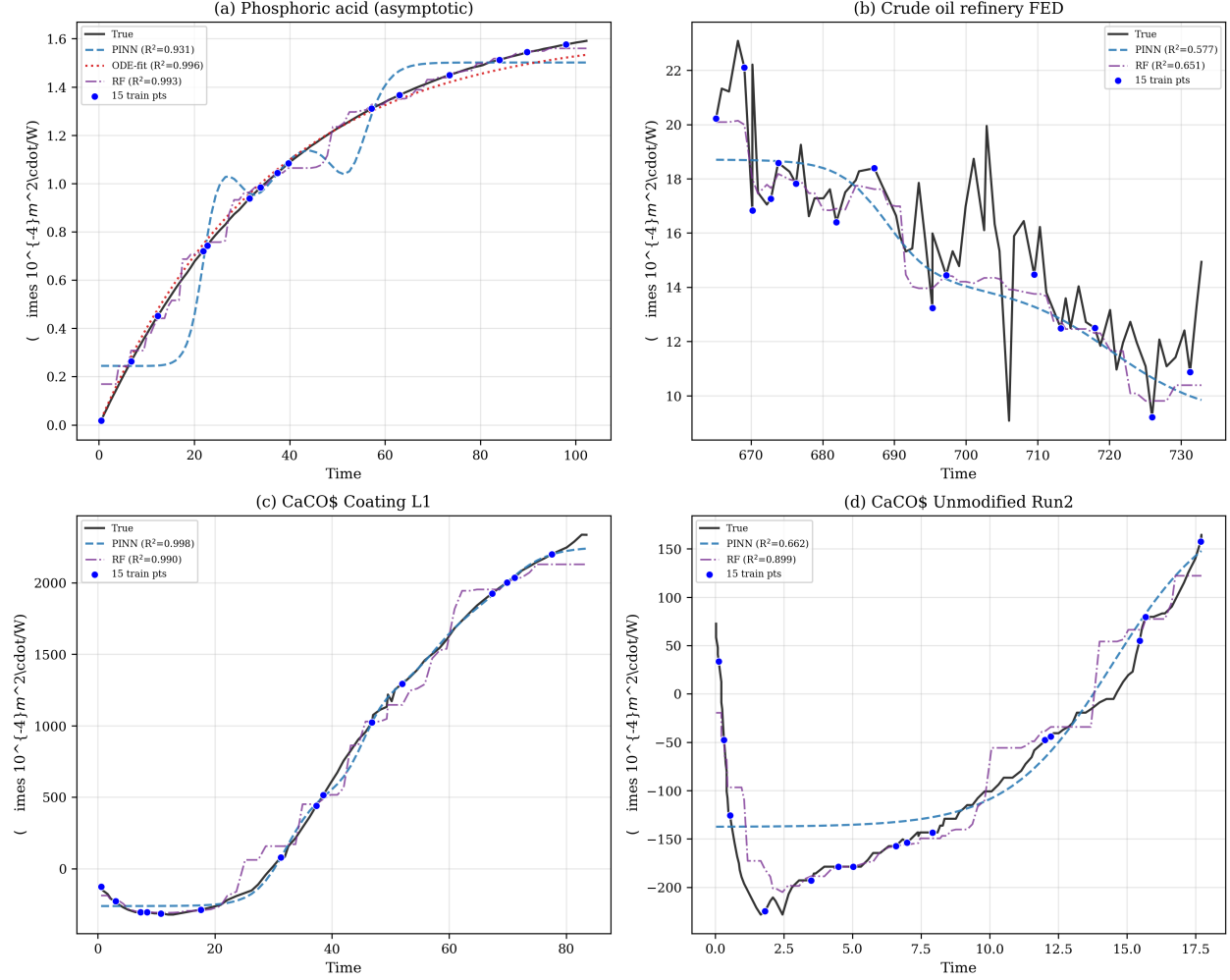
Figure 2: Representative prediction curves: true R_f(t) vs. PINN, ODE-fit, and RF predictions ( N = 15 sparse training points, seed=42). (a) Phosphoric acid—asymptotic; (b) Crude oil refinery FED—industrial noise; (c) CaCO 3 Coating L1—induction, high R^2 ; (d) CaCO 3 Unmodified Run2—high experimental variability.
