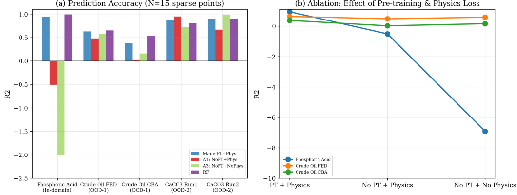
Figure 1: PINN Pre-training + Fine-tuning Performance on Real Fouling Curves
