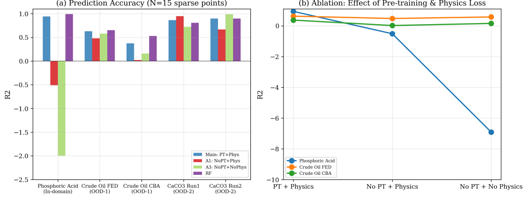
Figure 3: R^2 comparison across methods and sparsity levels. (a) Bar chart at N = 15 . (b) Ablation: pre-training vs. physics loss.
