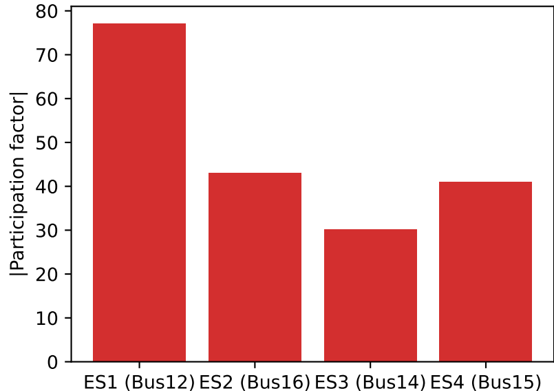
ES participation in inter-area mode
