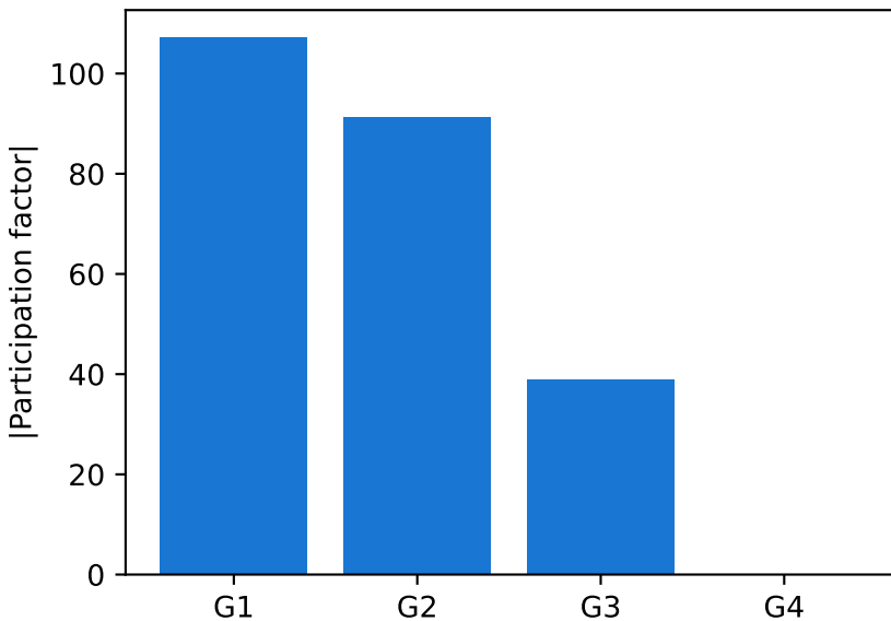
Inter-area mode ( f=0.579 Hz, \zeta=0.0245 )
