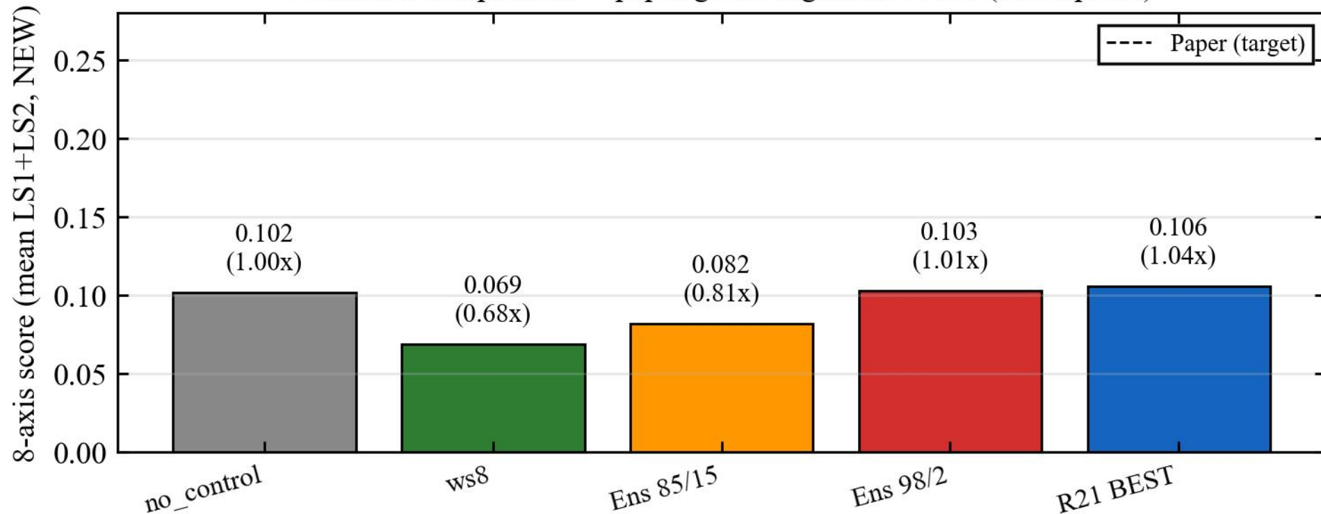
Controller comparison — paper-grade alignment scores (recomputed)
