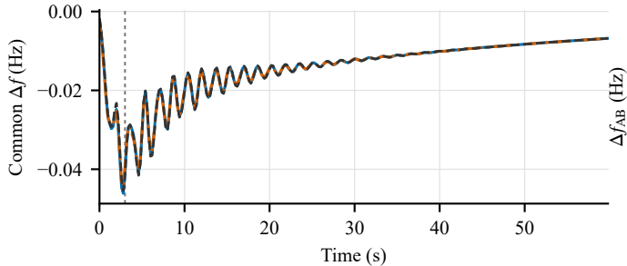
(a) Common frequency
