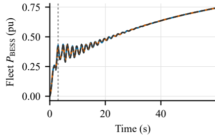
(e) Storage output
