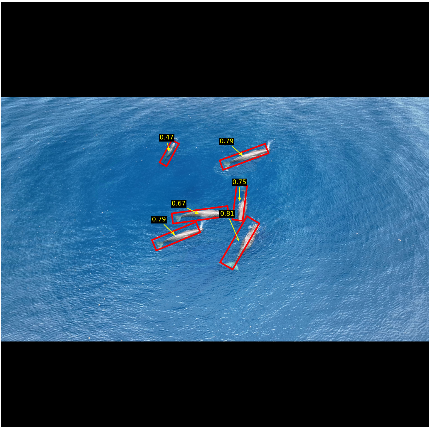
Whale Boxes With Confidence Scores
