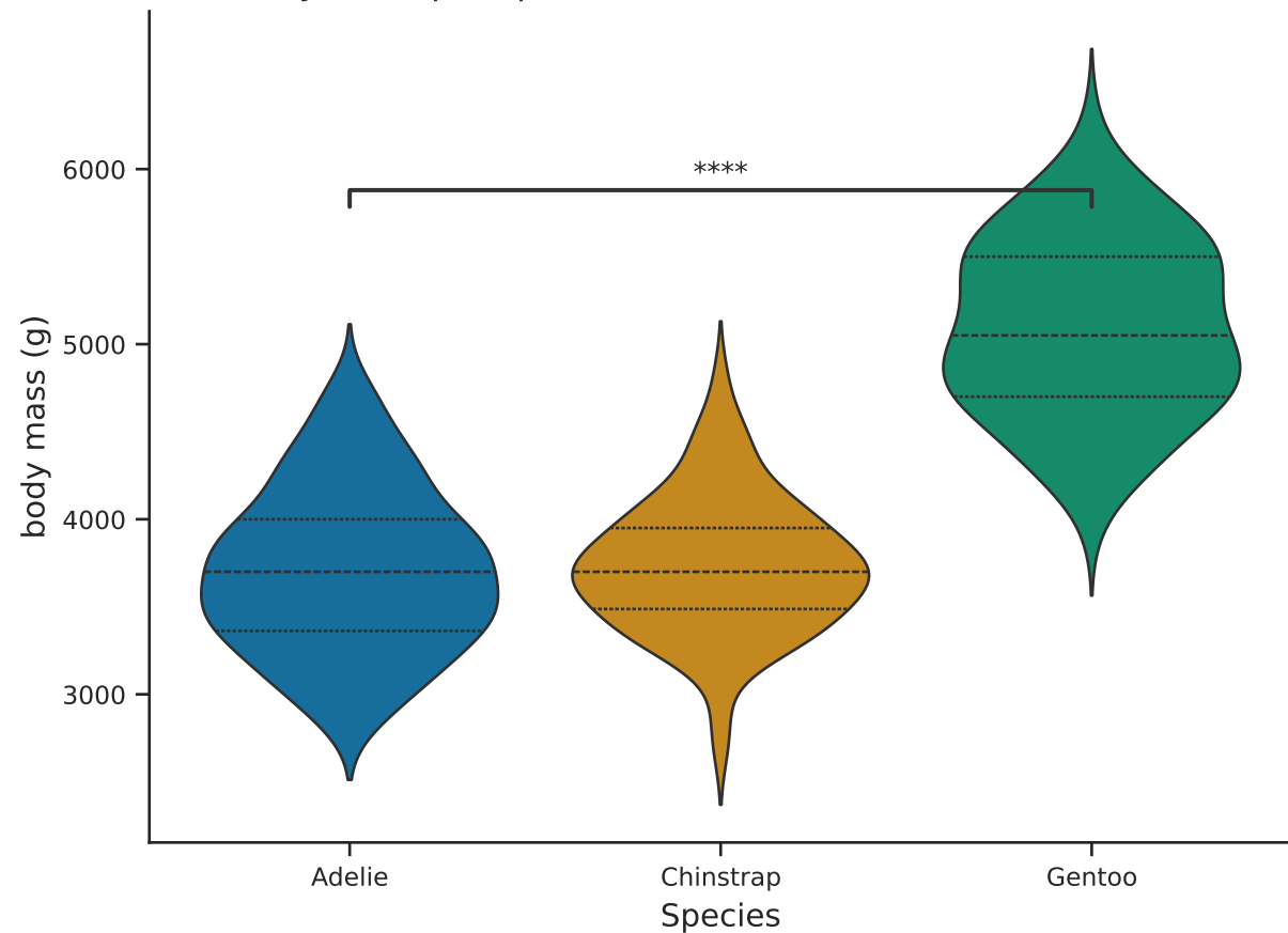
Body mass per species (Welch's t-test: Adelie vs Gentoo)
