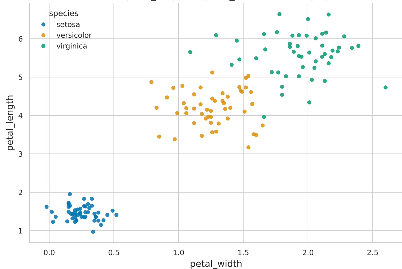
scatter of petal_length vs petal_width colored by species
