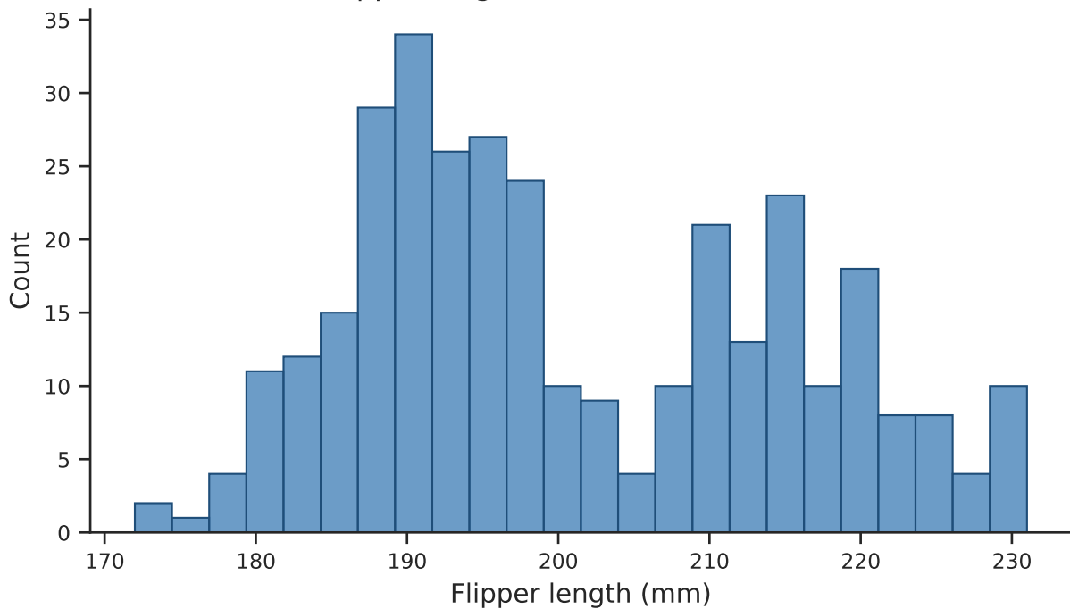
Flipper length — overall distribution
