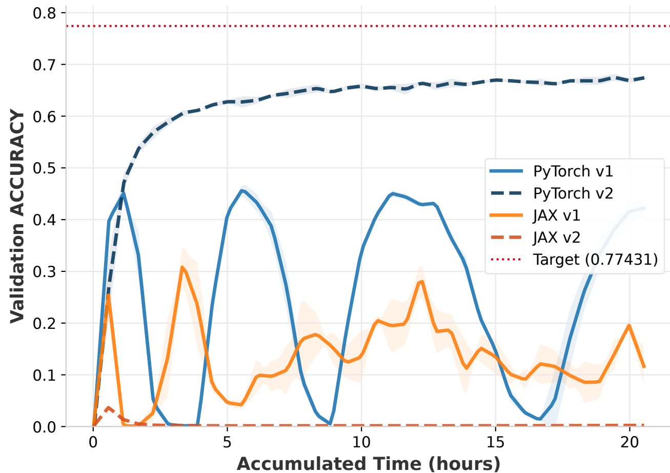
Workload: imagenet_resnet (Metric: accuracy)
