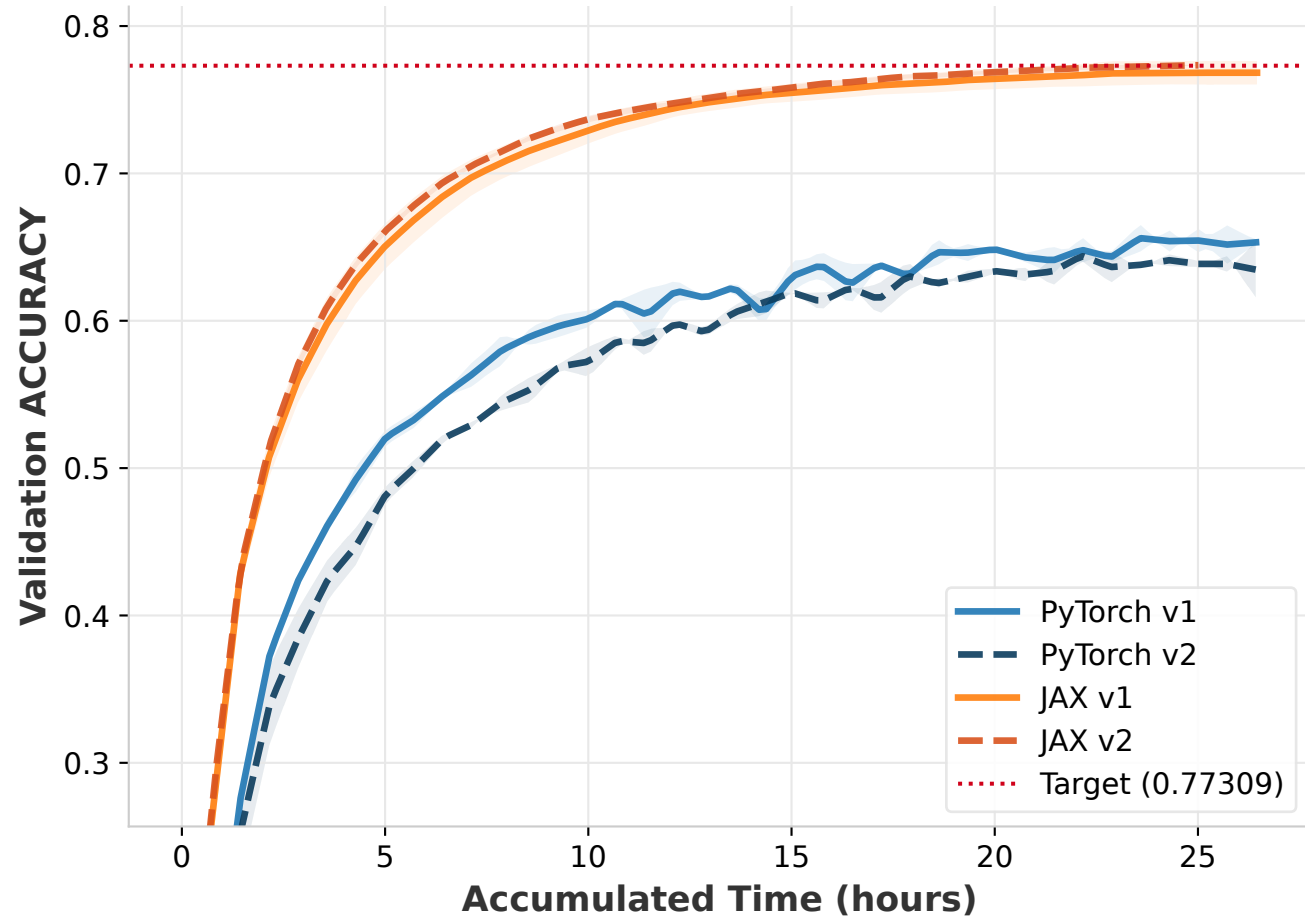
Workload: imagenet_vit (Metric: accuracy)
