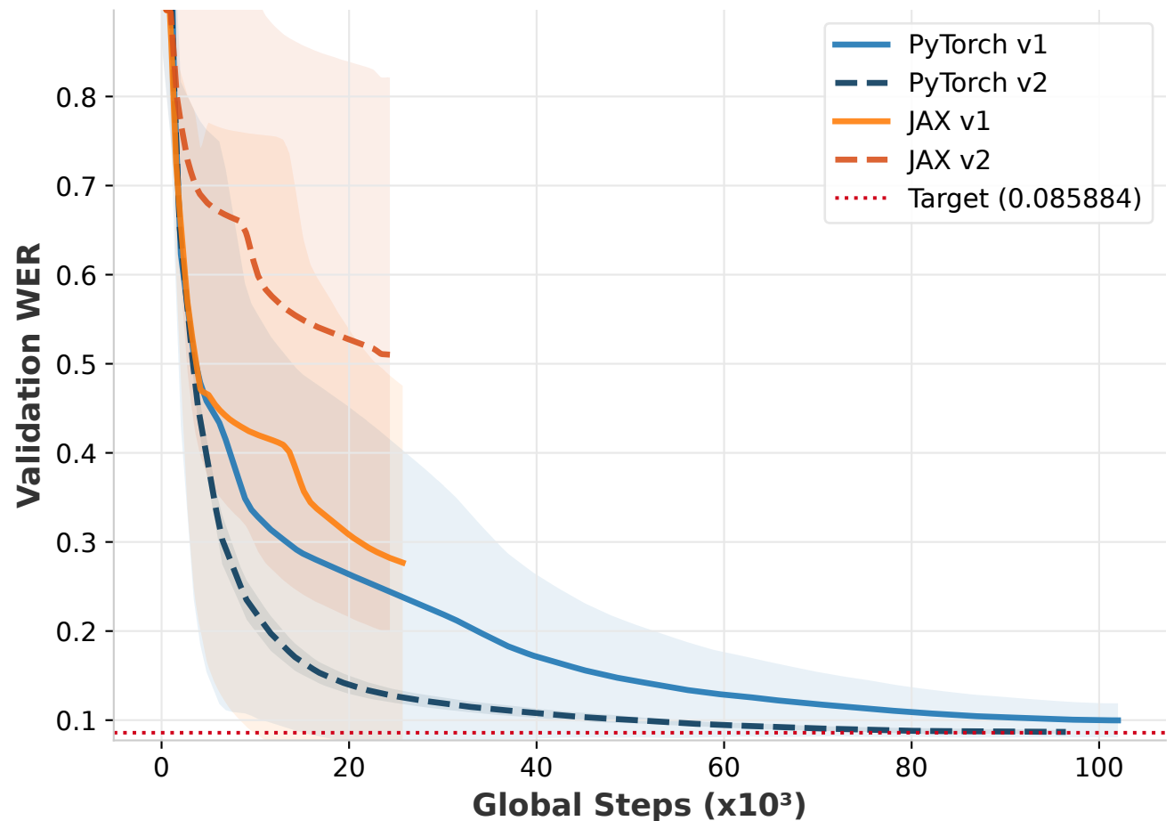
Workload: librispeech_conformer (Metric: wer)
