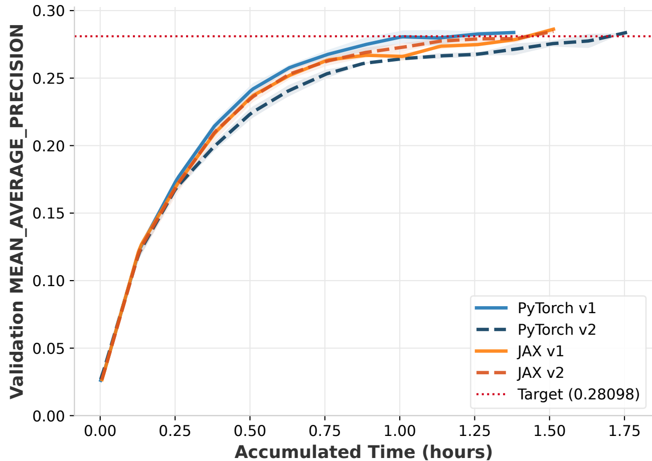
Workload: ogbg (Metric: mean_average_precision)
