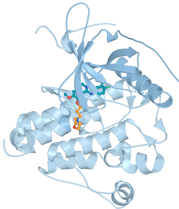
EGFR kinase domain
