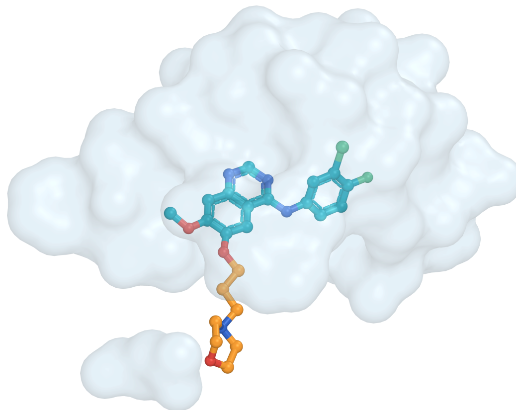
Crystallographic binding pose
