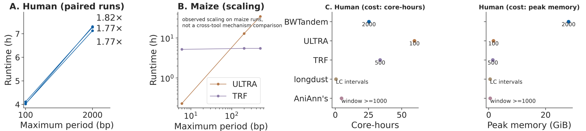
Supplementary Fig. S1. (A) Paired human range-cost measurements at commit 0363d8b: widening the maximum period from 100 to 2,000 bp gives ratios of 1.77-1.82 (mean 1.79), computed from per-arm elapsed seconds. (B) Observed maize ULTRA and TRF runtimes at their three period ceilings. (C) Human wall-time-based core-hour allocations and peak memory. These cross-tool observations differ in period range; the original ULTRA/TRF FASTA includes unplaced sequence, while the 2026 inputs match BWTandem's chromosome-only scope. BWTandem memory is the cgroup peak and the 2026 memory is GNU-time RSS. Sources: results/figures/paper_figs/data/fig2a_paired_runs.csv, fig2b_maize_scaling.csv and fig2c_human_cost.csv.
