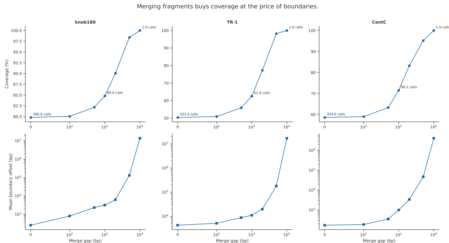
Supplementary Fig. S6. Coverage, boundary offset and calls per detected array after coordinate-only merging of the regenerated maize output. Gap zero already merges overlapping or touching calls and therefore differs from Supplementary Table S9’s raw-call offset baseline. Source: results/figures/paper_figs/data/figS2_postmerge.csv, derived from results/regen/maize_extra_evidence.json.
