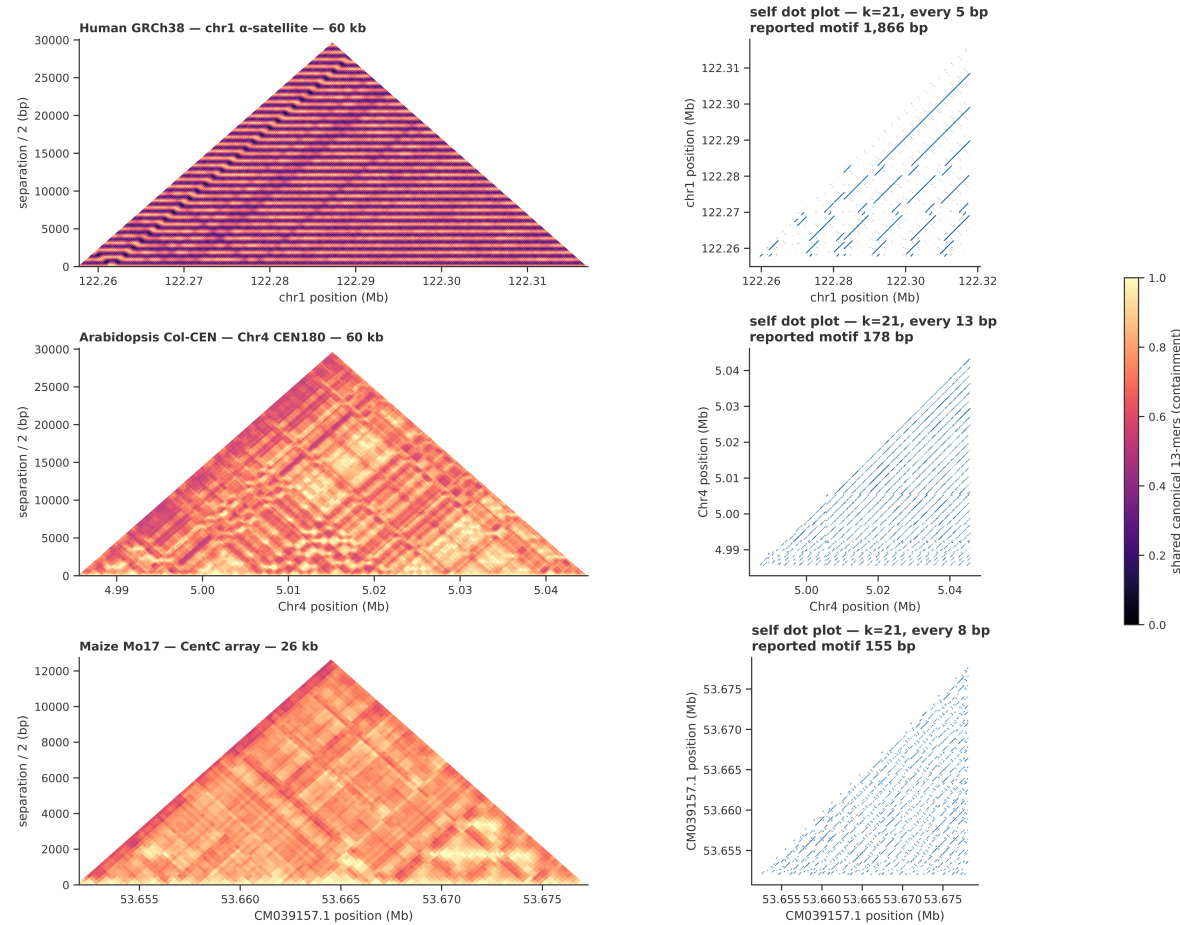
Supplementary Fig. S7. Self-similarity in three intervals drawn from deposited BWTandem calls: human chr1:122,257,803-122,317,803, Arabidopsis Chr4:4,985,644-5,045,644, and maize CM039157.1:53,652,014-53,678,133 (BED coordinates). The first two are 60 kb excerpts; the maize interval is the full 26,119 bp call. Their reported motif lengths are 1,866, 178 and 155 bp. Left: shared canonical 13-mer containment, |A \cap B| / \min(|A|, |B|) , between 1,000 bp windows sampled every 250 bp; this is a k-mer similarity statistic, not aligned nucleotide identity. Height is half the separation between window starts, so a feature at height h corresponds to separation 2h . Right: exact forward-strand 21-mer self matches sampled at the panel-specific strides. These are selected illustrations, not a systematic comparison of species or an independent validation of the reported motifs. Source: results/figures/paper_figs/plot_fig5_array_structure.py, whose REGIONS entries identify the FASTAs and intervals.
