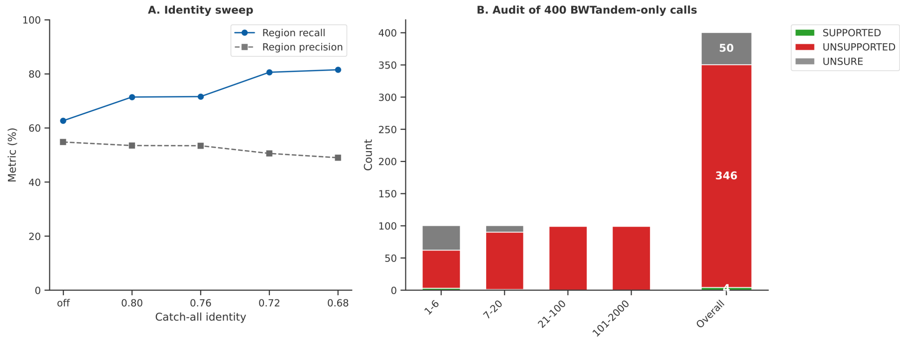
Supplementary Fig. S3. (A) The full-range identity sweep of Supplementary Section S2, evaluated on the catalog used to choose the operating point. (B) Single-reader verdicts for 100 calls per period stratum: 4 supported, 346 unsupported and 50 unsure. The 1.00% proportion is 4/400; excluding unsure calls gives 4/350, or 1.14%, with the descriptive Wilson 95% interval 0.45-2.90%. Equal sampling across strata does not make this a population-weighted estimate. Sources: results/figures/paper_figs/data/fig3a_idsweep.csv and fig3b_audit.csv.
