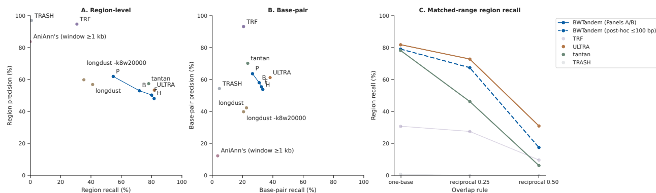
Fig. 2. Native-period-100 operating points (A–B) and reciprocal-overlap sensitivity of post-filtered full-range output (C). The 2026 points in A–B are full-range, not band-matched. Original Figure 1 and its complete caption are preserved as Supplementary Figure 1.
