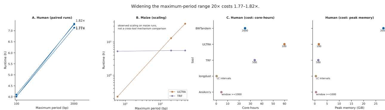
Fig. 1. Paired human range cost (A); separate maize runtime (B) and human core-hour/memory observations (C). Cross-tool ranges, FASTA scopes and memory accounting differ. Original Figure 2 and its complete caption are preserved as Supplementary Figure 2.
