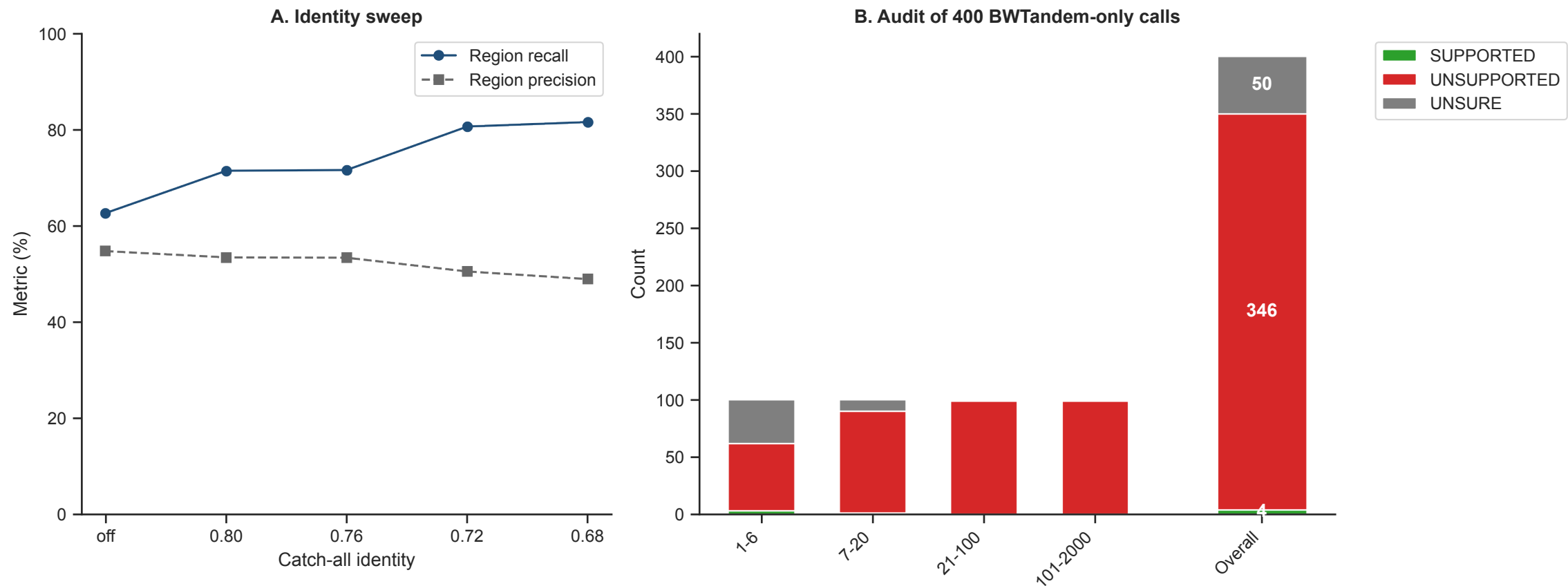
Figure 3. (A) Precision–recall trade-off for the catch-all identity sweep (Supplementary Table S3). (B) Blinded manual audit of 400 BWTandem-exclusive calls (100 per period stratum). Results show 4 supported, 346 unsupported, and 50 unsure calls (Wilson 95% CI: 0.4–2.9% for definitive verdicts).
