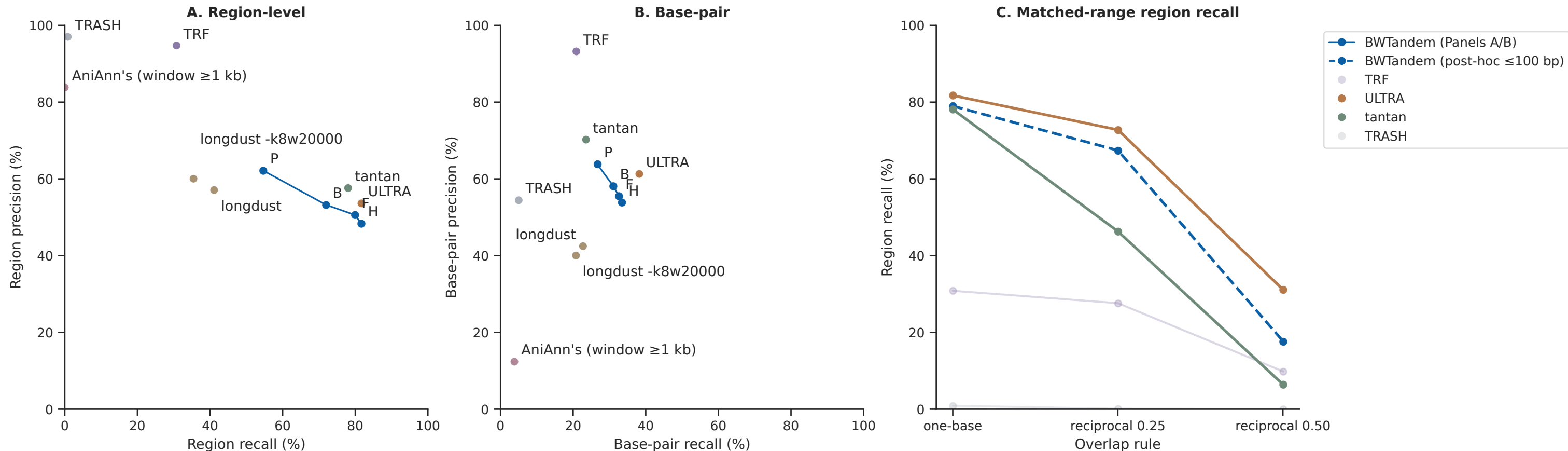
Figure 1. (A) Region-level and (B) base-pair precision-recall on GRCh38 against the adotto catalog (one-base overlap). BWTandem's four configurations (P, B, F, H) are connected lines; competing tools are single points. (C) Region recall evaluated only for periods \leq 100 bp across three overlap rules. ULTRA performs best, with BWTandem second. BWTandem data in (C) uses full-range output filtered post-hoc to \leq 100 bp to ensure accurate boundary assessment. Reciprocal rules here stress-test boundary precision against a merged catalog rather than absolute ranking. The 2026 tools are excluded from (C) as they lack period bounds. Panels A and B plot the four native --max-period 100 operating points (Table 1d), where F reads 79.88% region recall; panel C plots the post-hoc filtered arm, which is what Table 1b reports, at 78.87%.
