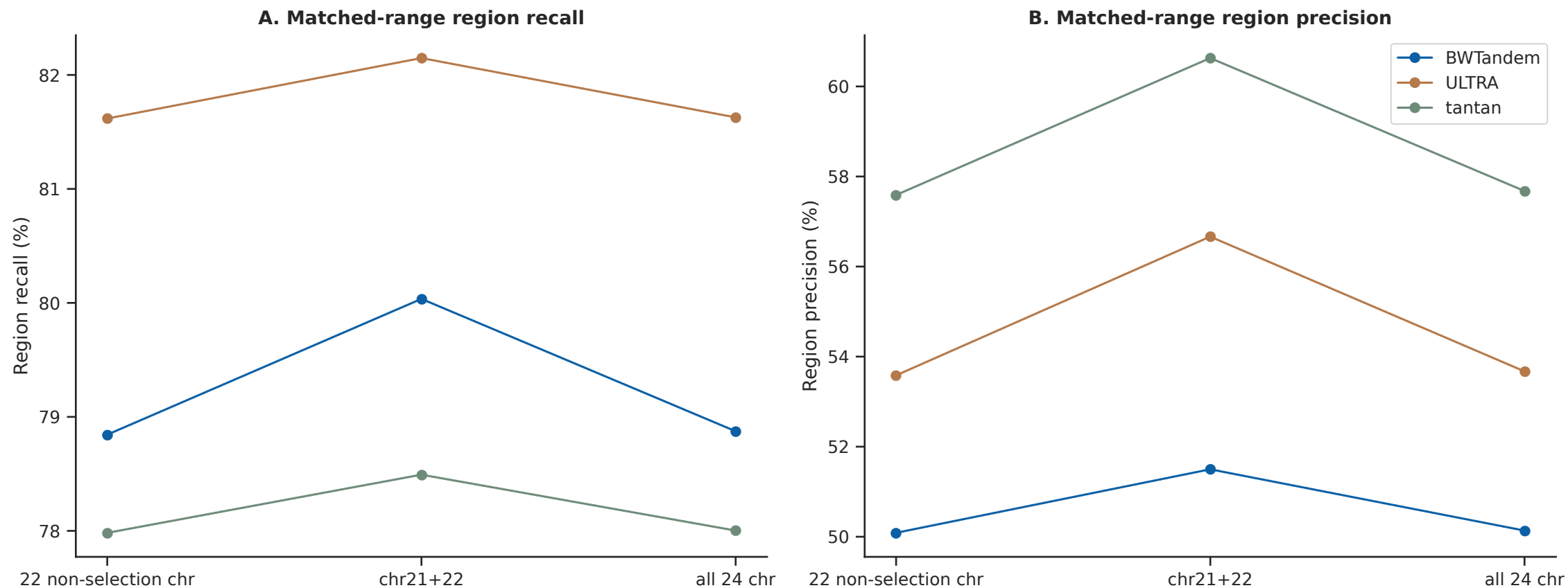
Figure S1. Matched-range region recall (A) and precision (B) on the 22 non-selection chromosomes, the 2 selection chromosomes, and all 24.
