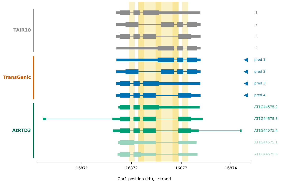
(B) AT1G44575 — TransGenic reproduces the alternative transcripts shared by TAIR10 and AtRTD3
