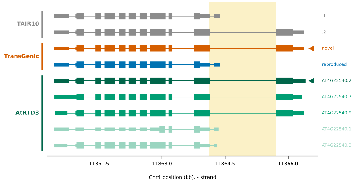
(D) AT4G22540 — TransGenic predicts an AtRTD3-supported isoform absent from TAIR10
