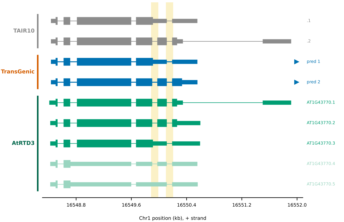
(A) AT1G43770 — TransGenic reproduces the alternative transcripts shared by TAIR10 and AtRTD3
