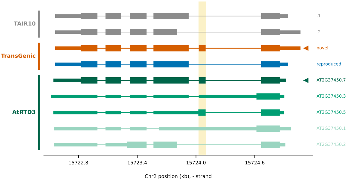
(C) AT2G37450 — TransGenic predicts an AtRTD3-supported isoform absent from TAIR10
