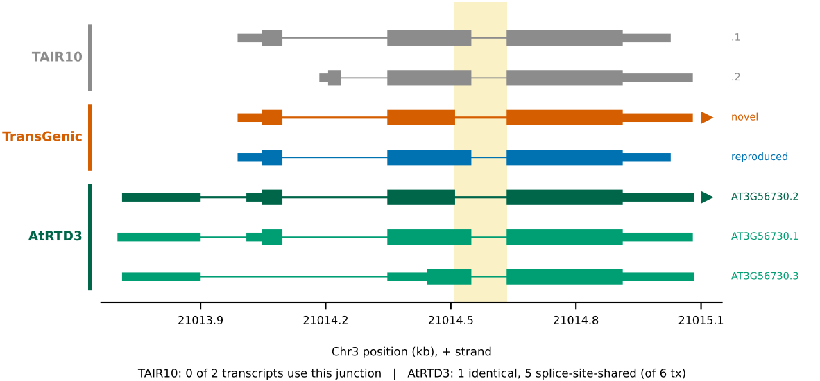
(E) AT3G56730 — TransGenic predicts an AtRTD3-supported isoform absent from TAIR10
