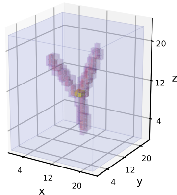
ref3+U-Net
