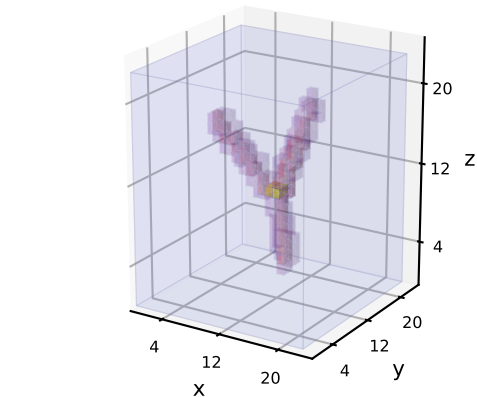
GT
