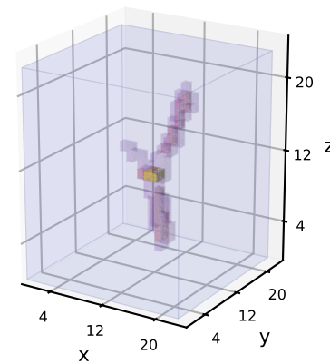
U-Net residual
