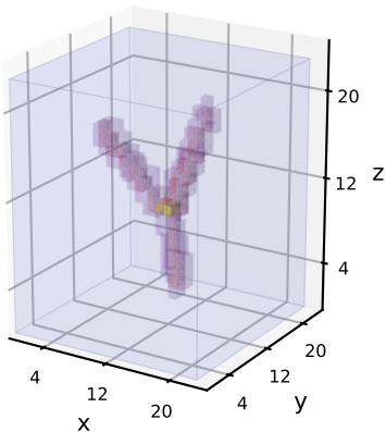
GT
