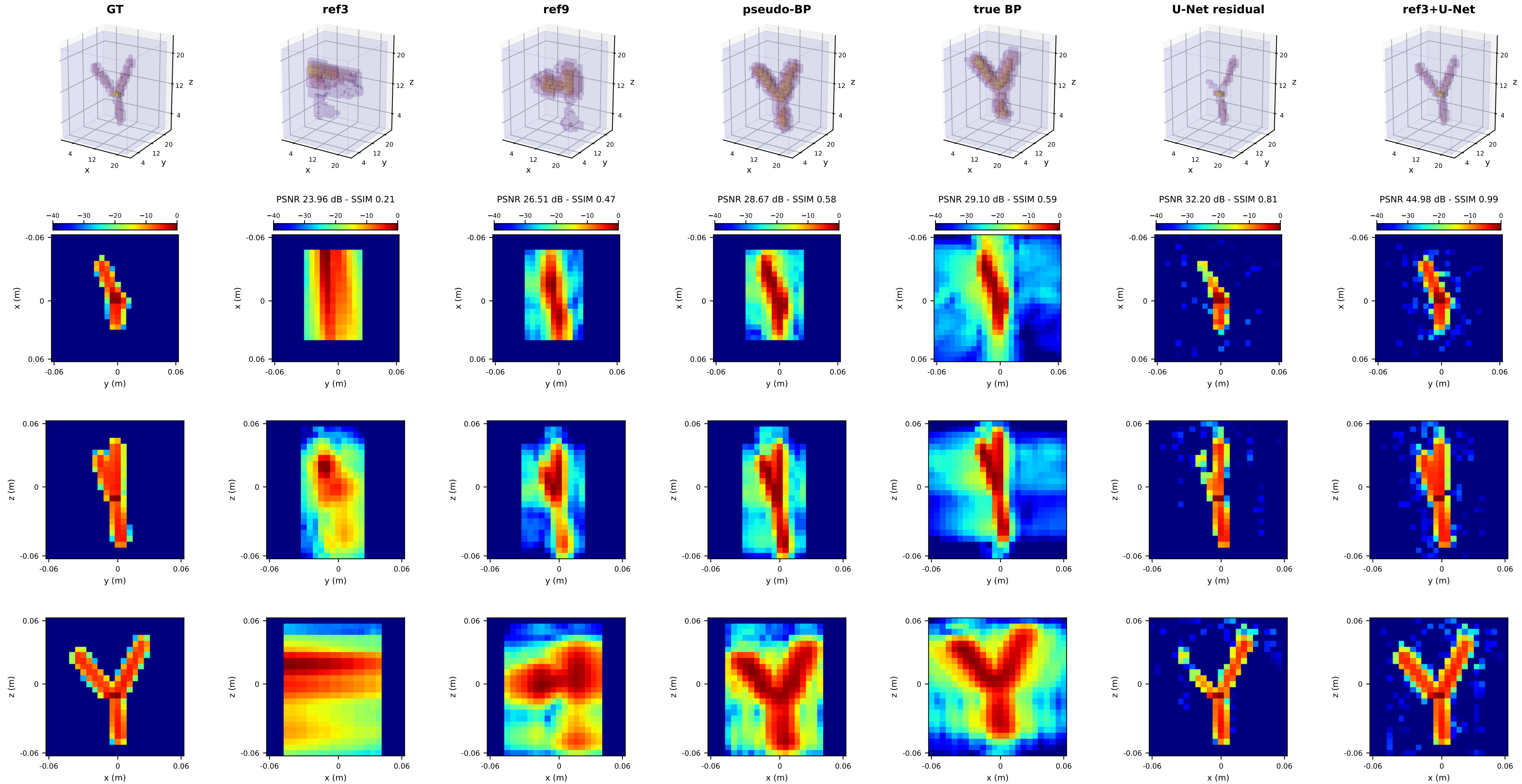
Dense-volume Y target: pseudo-BP versus true BP
