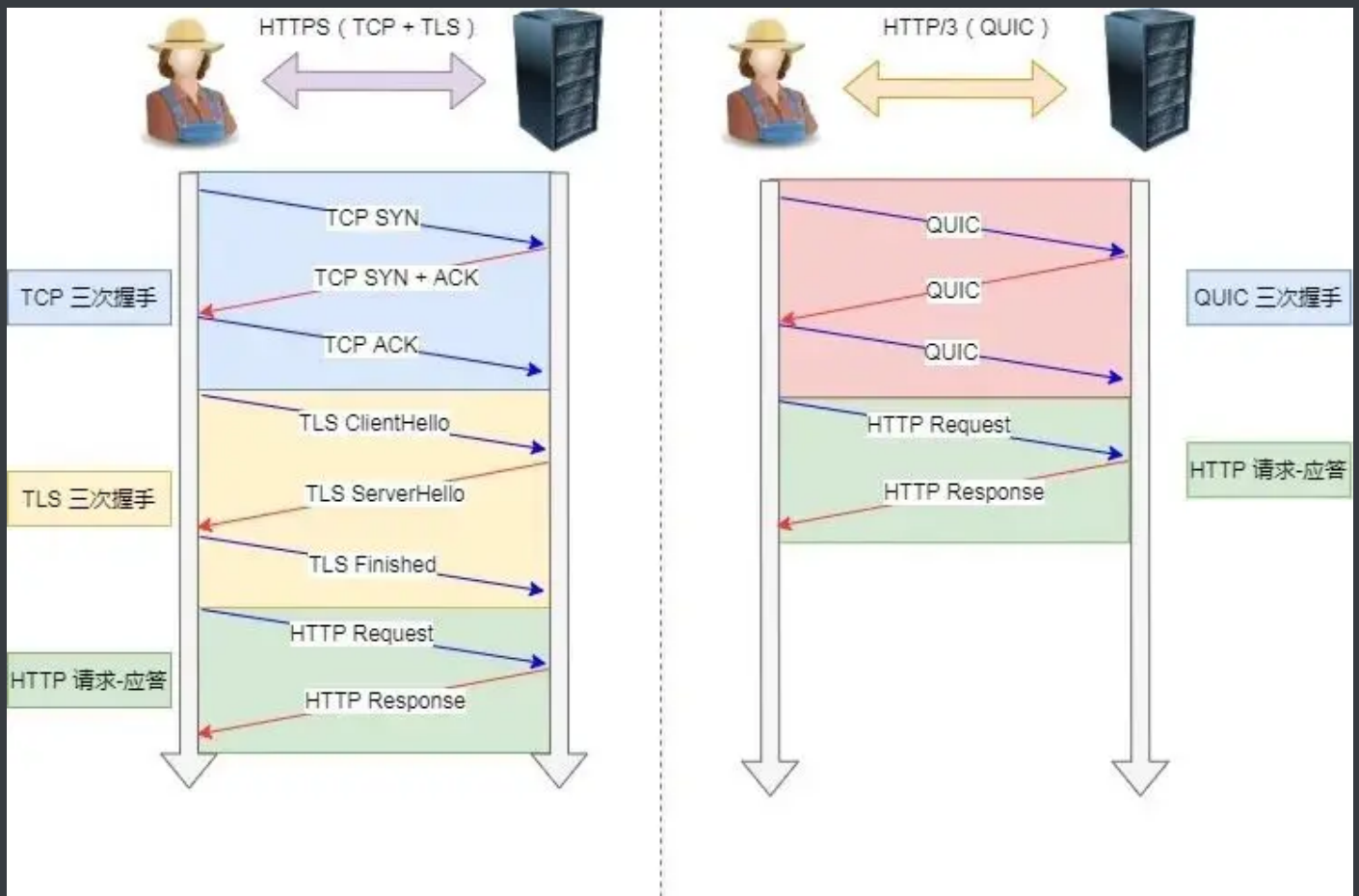
TCP HTTPS (TLS/1.3) 和 QUIC HTTPS
