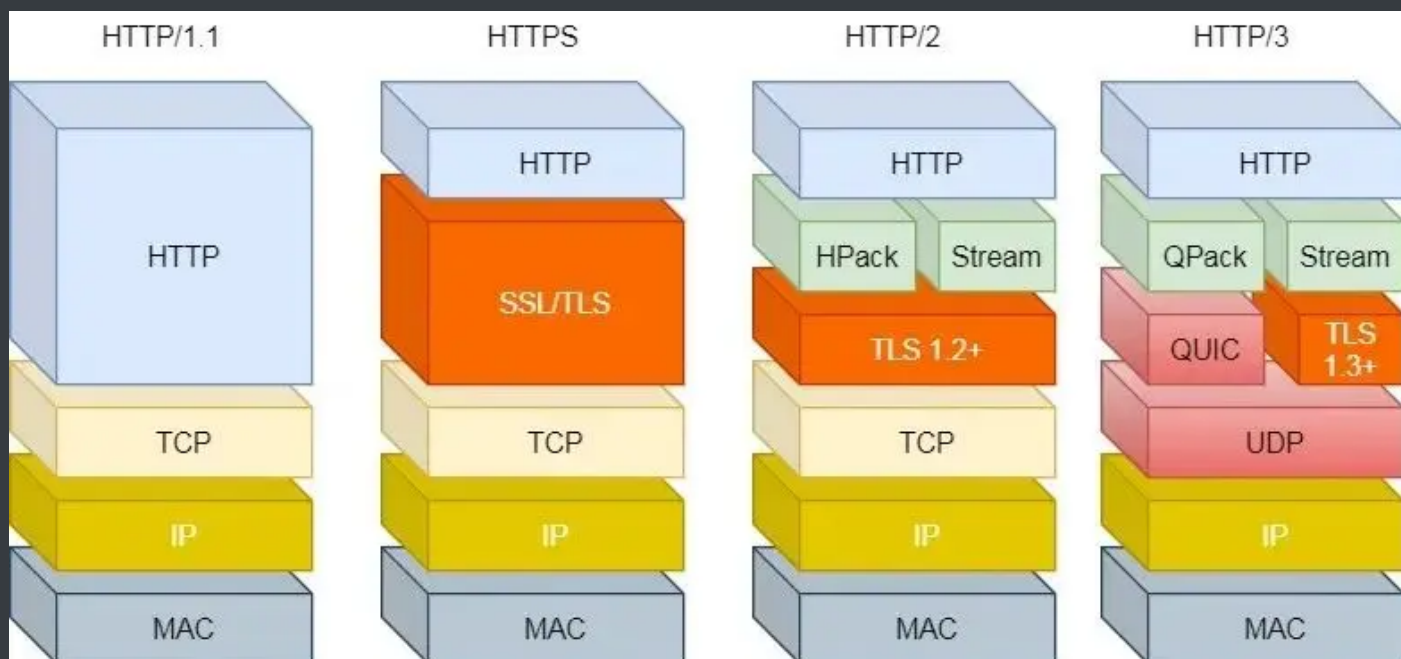
HTTP/1 ~ HTTP/3
