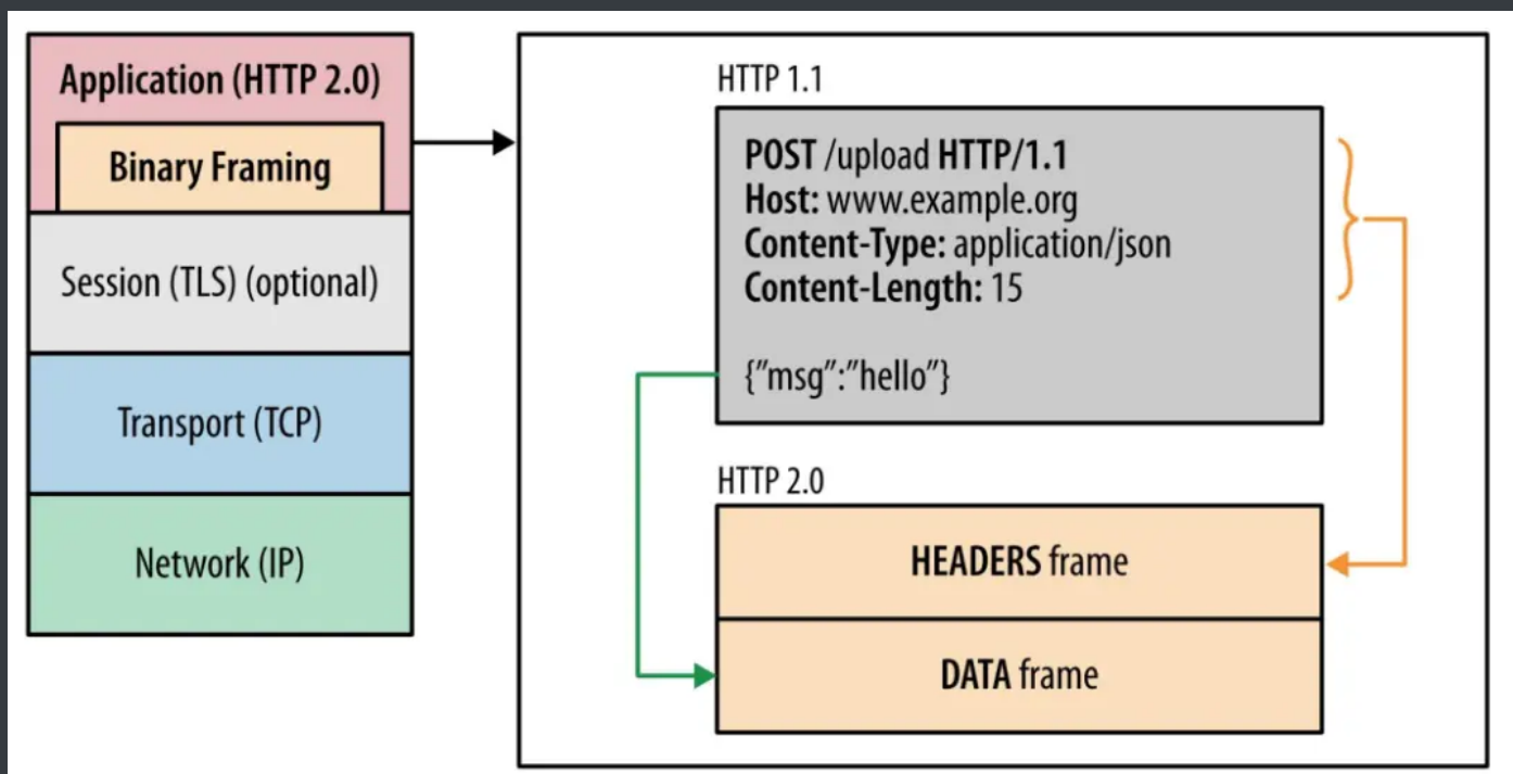
HTTP/1 与 HTTP/2
