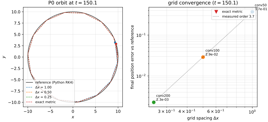
Figure 3: Grid convergence of the P0 circular orbit over one period ( t = 150.1 M ). Left: orbit traces in the x - y plane for the interpolation runs ( \Delta x = 1.0, 0.5, 0.25 ) and the exact-metric run, compared with the independent Python reference (solid). Right: final-position error versus grid spacing (markers), with a reference line of the measured order 3.7 (dotted).
