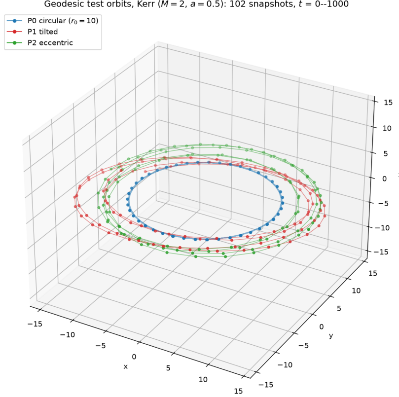
Figure 1: The three test orbits of Table 1 in the Kerr spacetime ( M = 2 , a = 0.5 ), integrated by the thorn in Exact mode over T = 1000 M (102 snapshots). P0, a circular orbit of radius r = 10 in the equatorial plane (blue); P1, P2’s orbit given a small vertical kick, precessing out of the plane (red); P2, an eccentric orbit with r_a = 15 , r_p = 12.03 (green).
