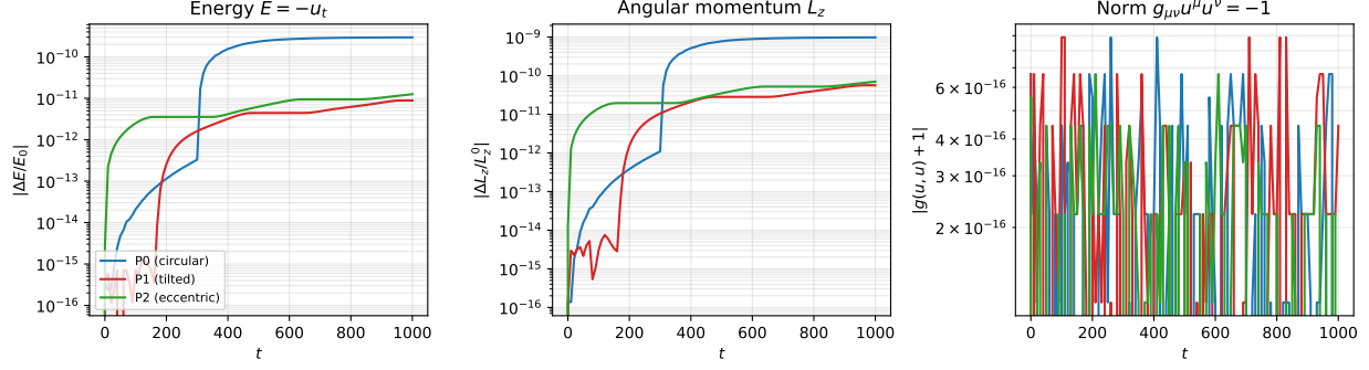
Figure 2: Conservation over T = 1000 M (Exact mode): relative drift of the energy E (left) and axial angular momentum L_z (middle), and the norm residual |g_{\mu\nu}u^\mu u^\nu + 1| (right), for the three orbits of Table 1. All quantities are conserved at the \lesssim 10^{-9} level.
