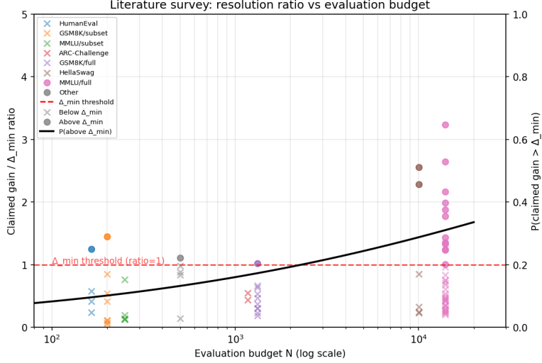
Fig. 4 Literature survey scatter plot: ratio of claimed gain to \Delta_{\min} vs. evaluation budget N (log scale). Points above the red dashed line (ratio > 1 ) correspond to claims where the reported improvement exceeds the minimum detectable gap. The black curve shows a logistic regression fit (probability that a claim is resolvable). Marker shape indicates resolvability (circles = above threshold, crosses = below). Colors denote benchmark categories.
