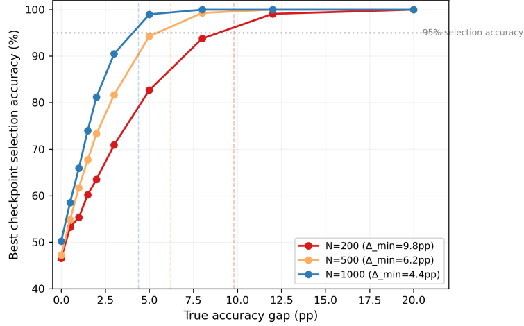
Fig. 1 Synthetic validation: selection accuracy vs. true gap for N \in \{200, 500, 1000\} . Dashed lines mark \Delta_{\min} .
