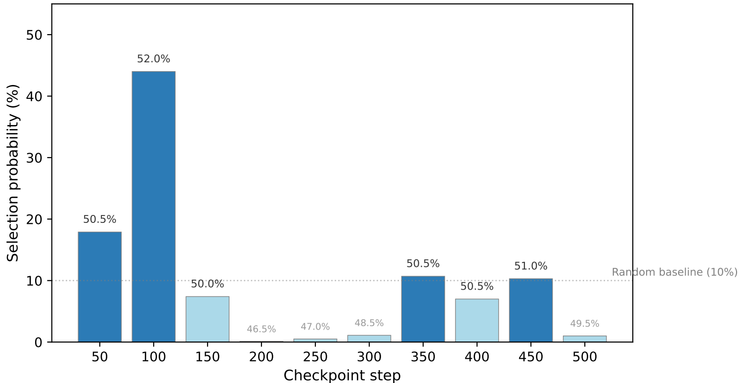
Bootstrap checkpoint selection distribution (N=200, 10,000 resamples)
