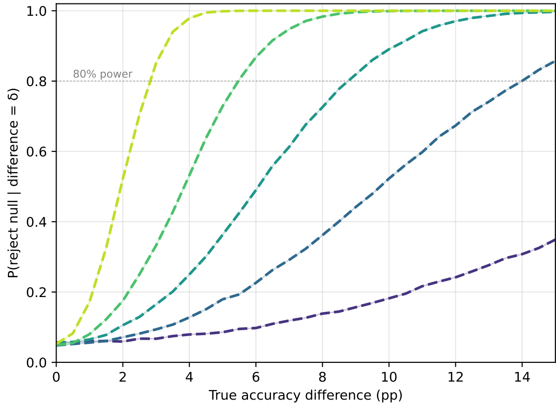
(b) Power curves (dashed) with resolution rate (faint)
