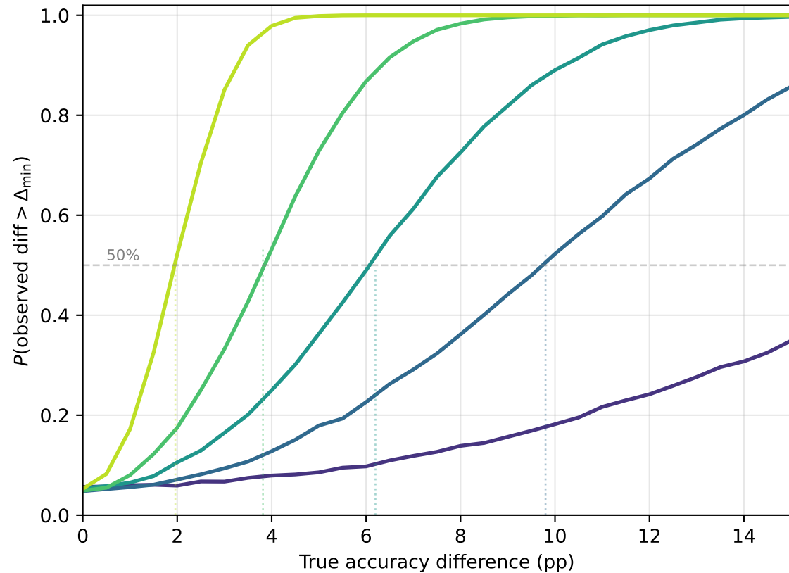
(a) Resolution rate by evaluation budget
