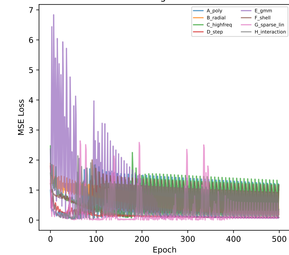
Training curves
