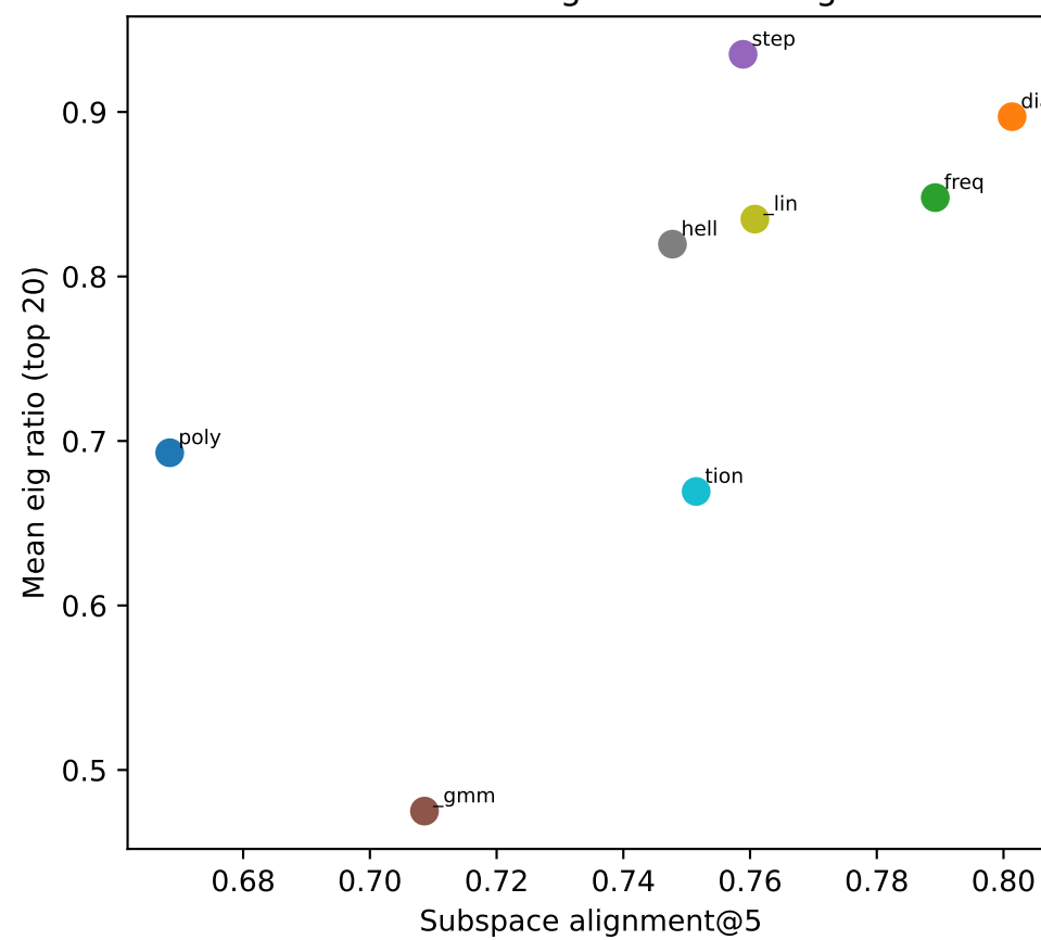
Rotation vs eigenvalue change
