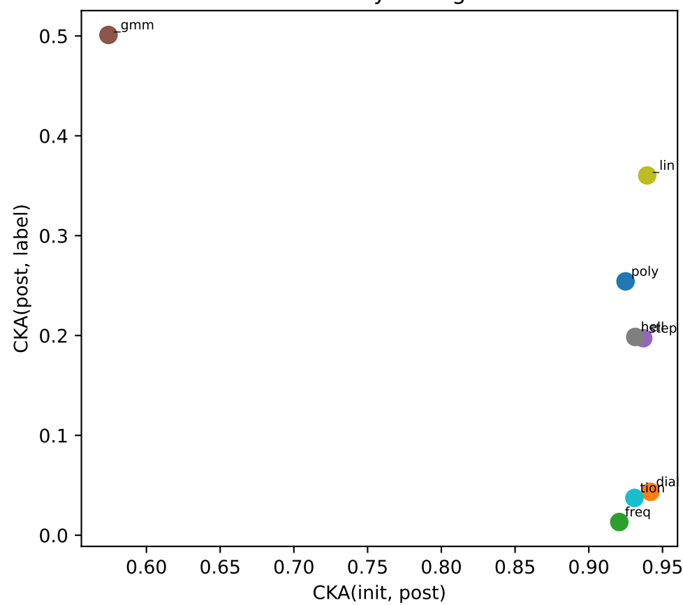
Kernel stability vs alignment
