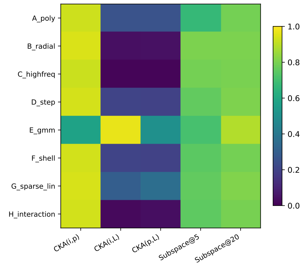
Kernel stability vs alignment
