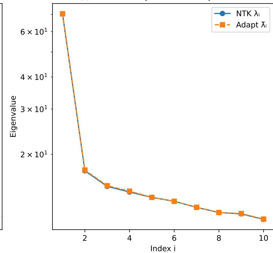
(f) NTK vs Adaptive Kernel Spectrum
