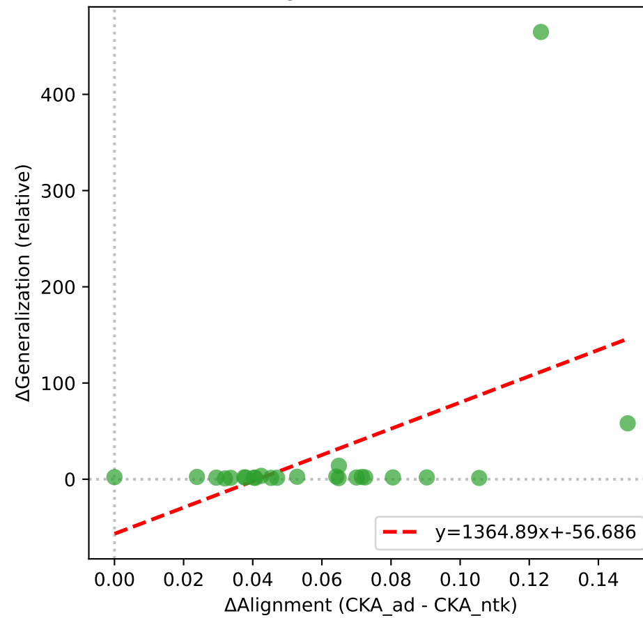
(e) \Delta\text{Align} vs \Delta\text{Gen} R^2=0.231
