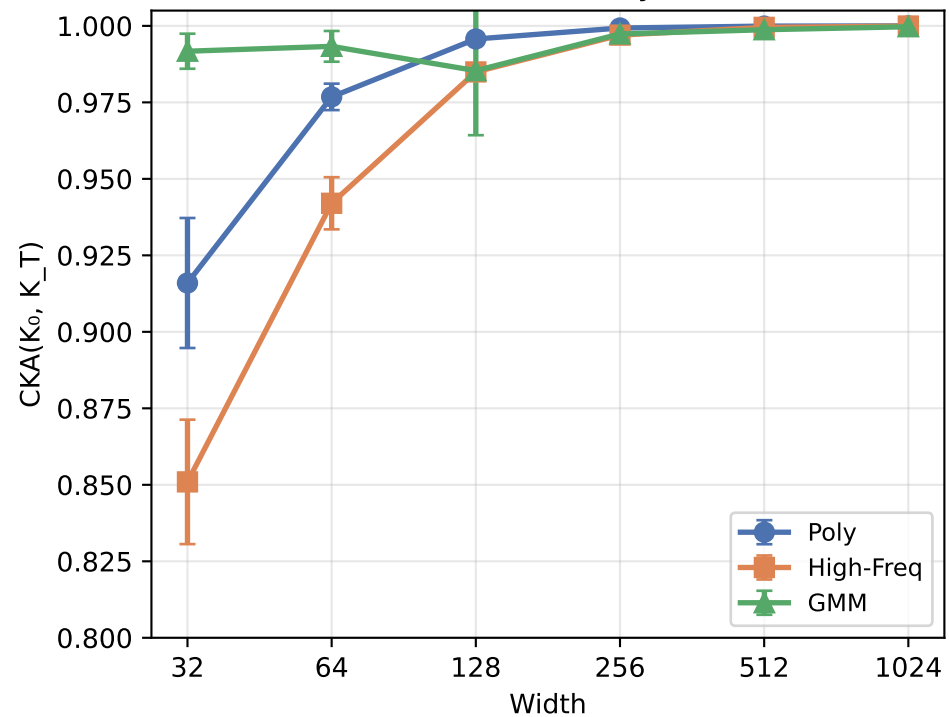
(a) Kernel Similarity (CKA)
