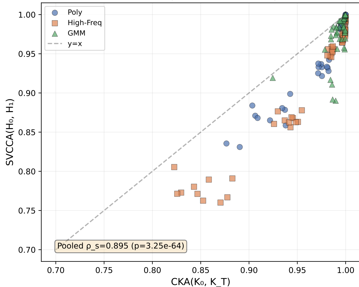
CKA vs SVCCA: Representation Similarity Metrics
