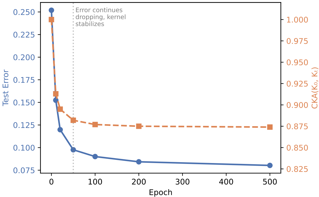
Poly width=32: Error decreases while kernel stabilizes
