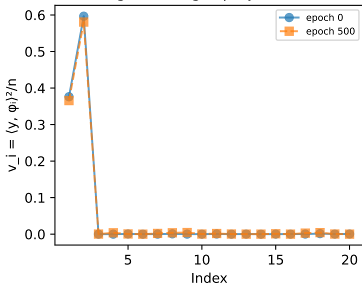
gmm: Target projection
