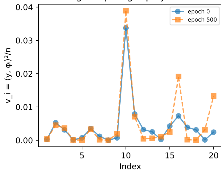
gmm: Target projection
