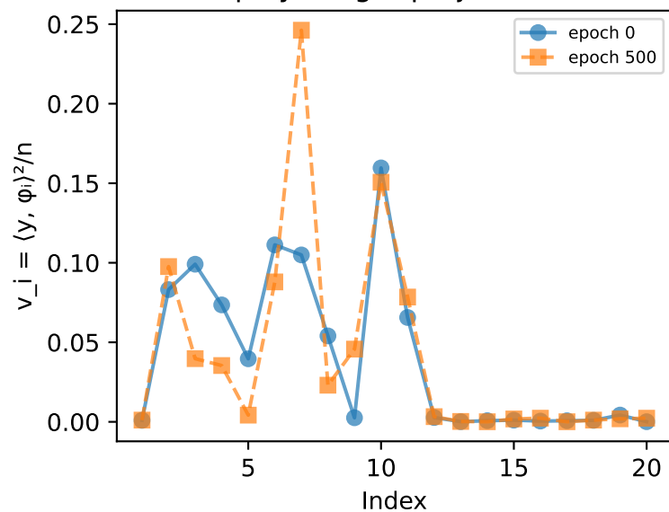
highfreq: Target projection
