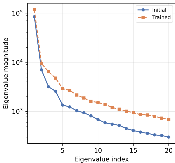
CNN W=128 on CIFAR-10
