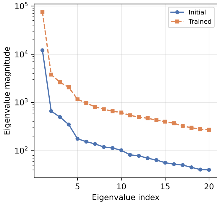
CNN W=16 on CIFAR-10
