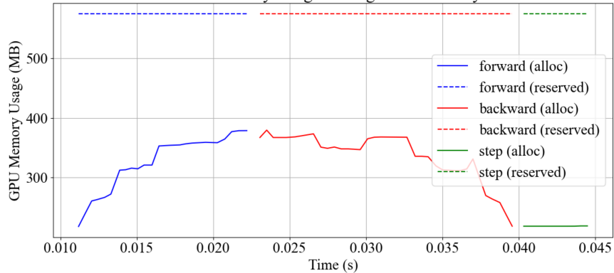
GPU Memory Usage During One TGN Layer
