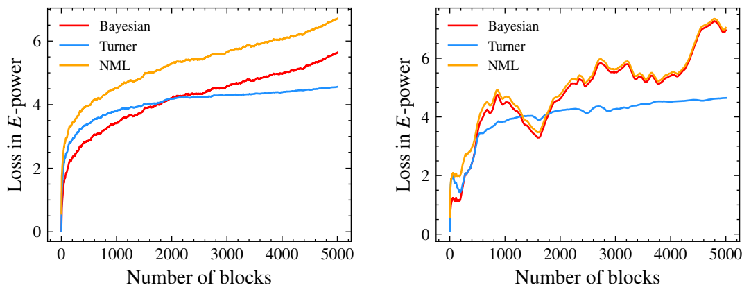
(a) Fixed mean (\theta_a, \theta_b) = (0.6, 0.4) for Bernoulli stream, group size are fixed as 5.
