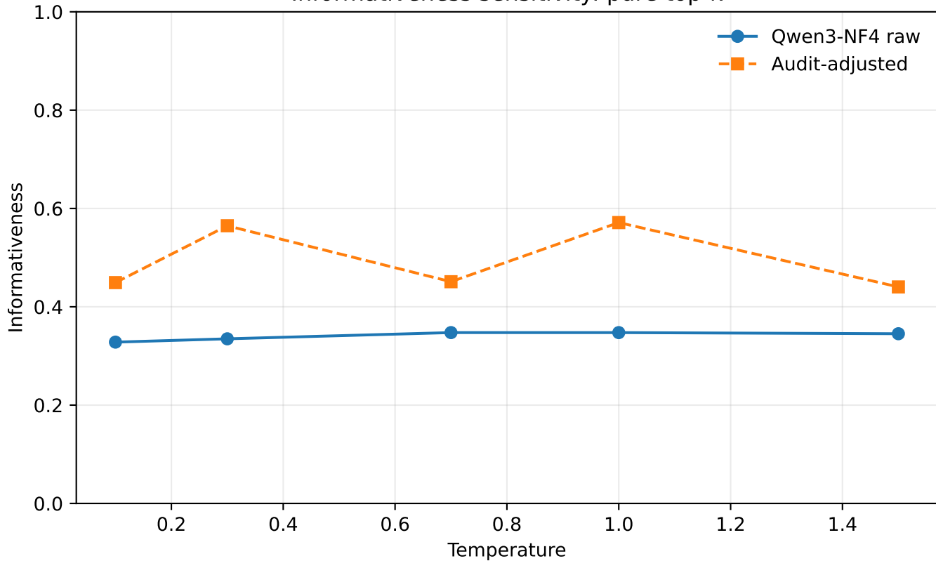
Informativeness sensitivity: pure top-k
